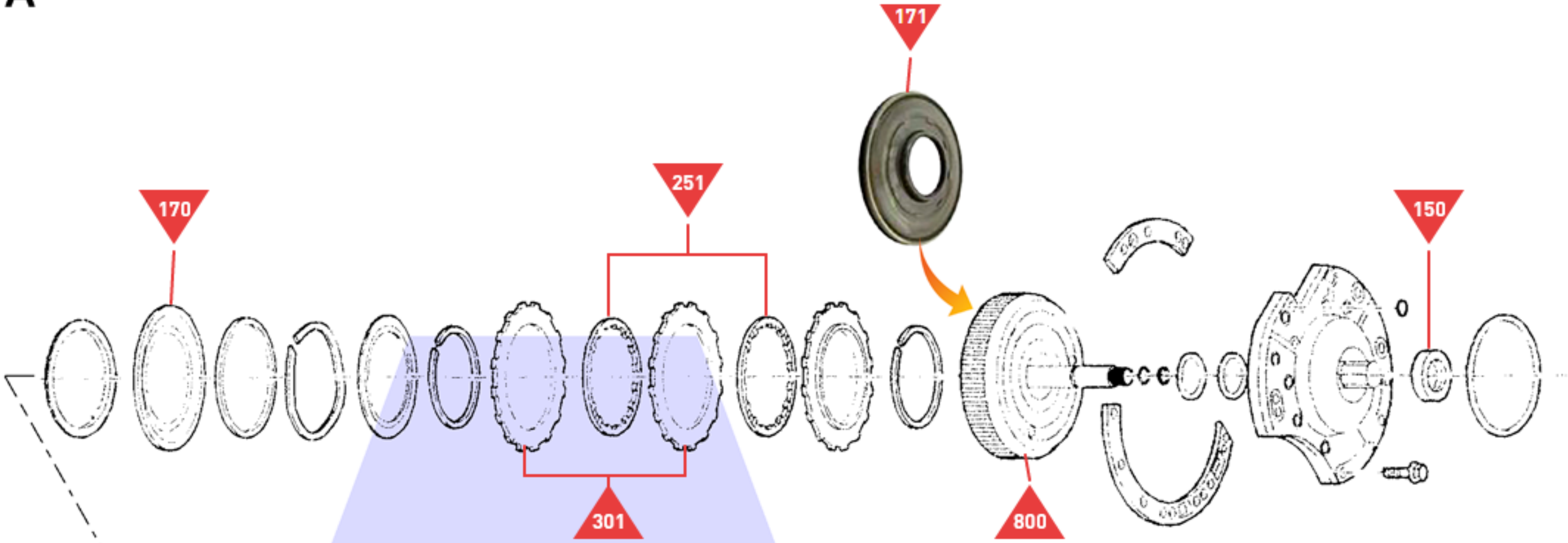
Front Pump Assy, Planetary, Forward and Reverse Clutches
