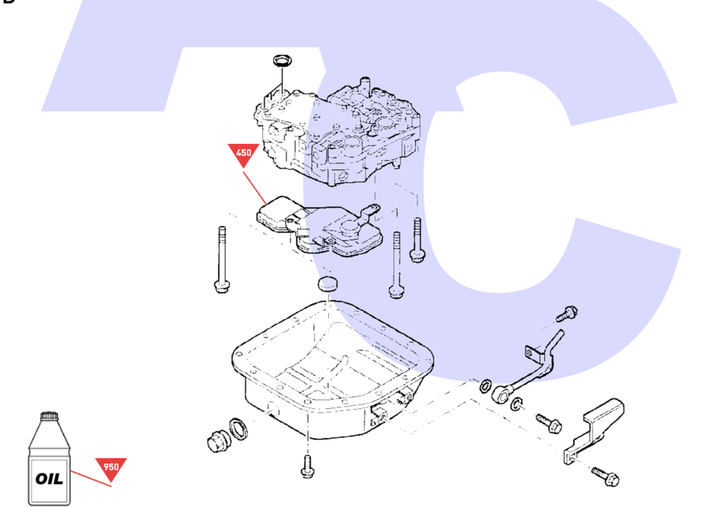
Valve Body, Filter and Oil Pan
