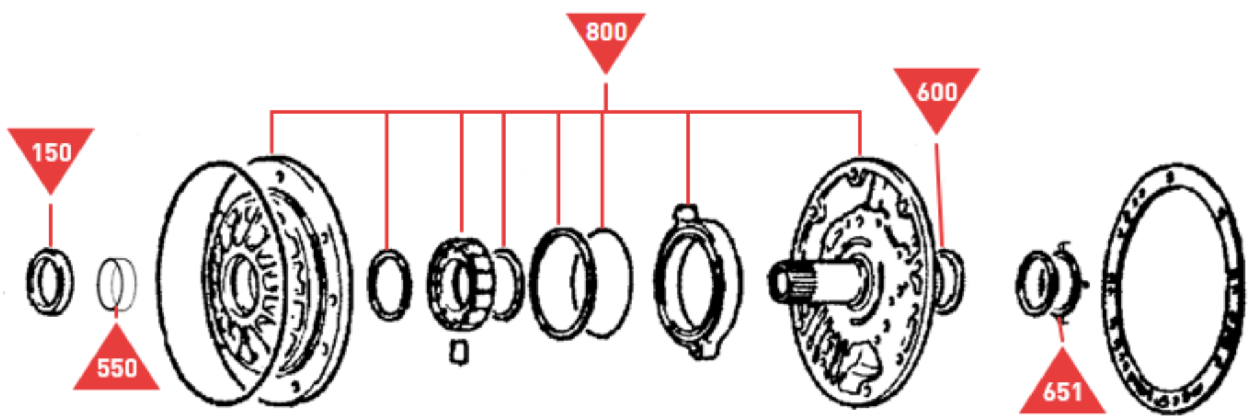
Oil Pump
