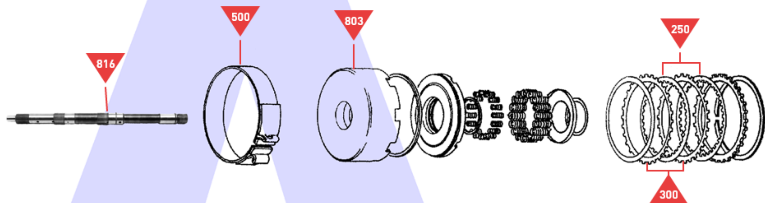
Reverse Clutch
