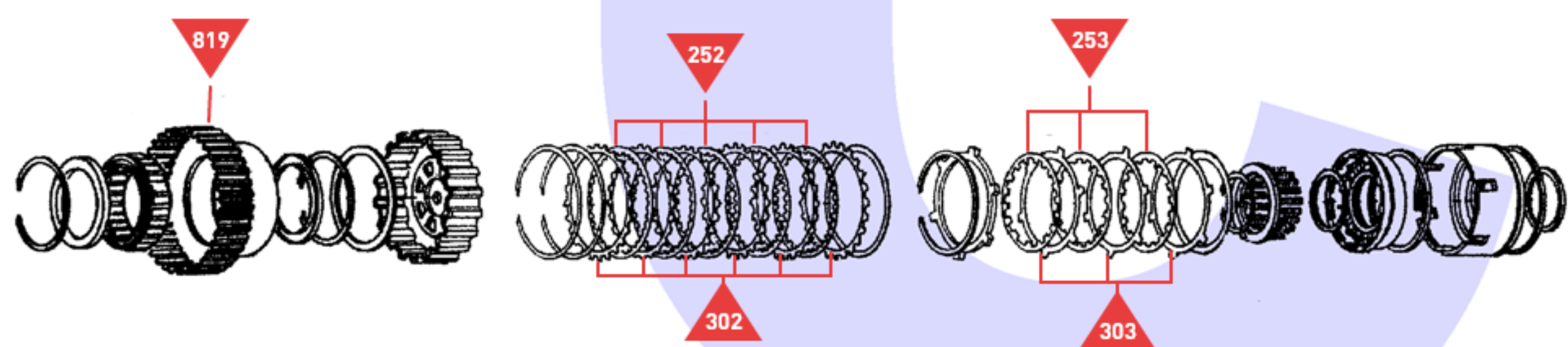
Forward & Overrun Clutches
