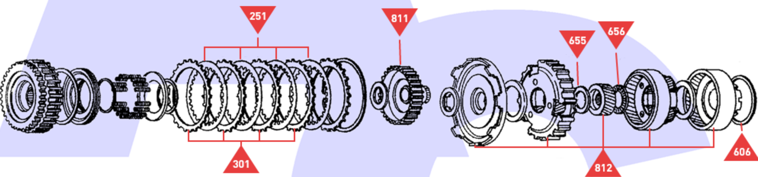
High Clutch & Planetary Set
