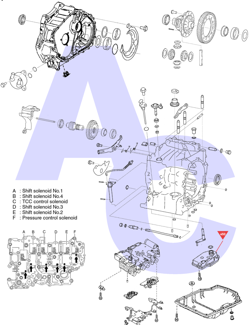
Bell Housing, Differential, Secondary Gear, Main Case, Linkage, External Components Valve Body, Filter & Oil Pan
