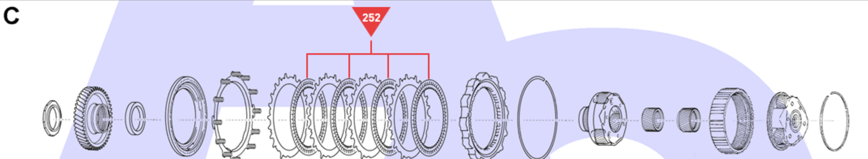
Low Clutch, Input Shaft, High Clutch Hub & Low Clutch Hub
