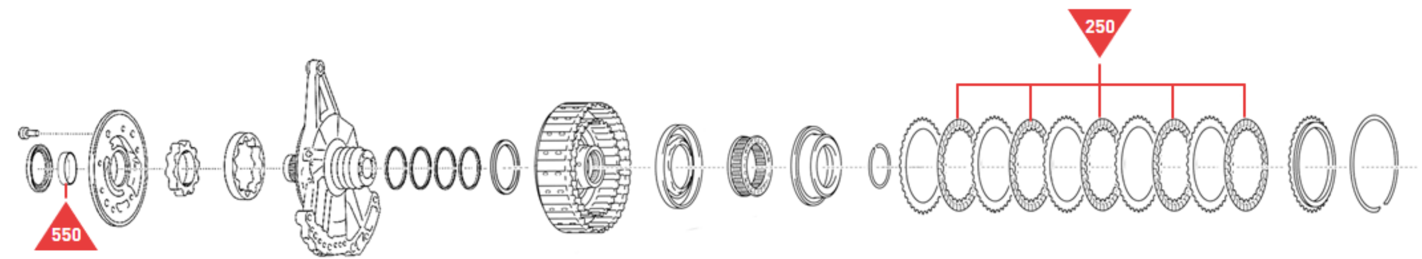
Oil Pump & High Clutch
