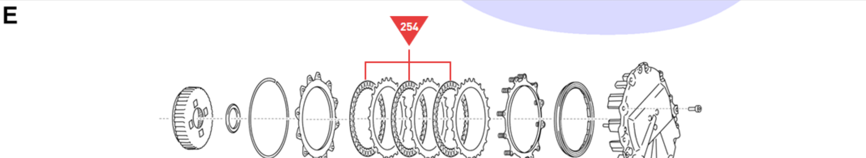
Reaction Sun Gear, Reaction Planetary & 2-6 Brake
