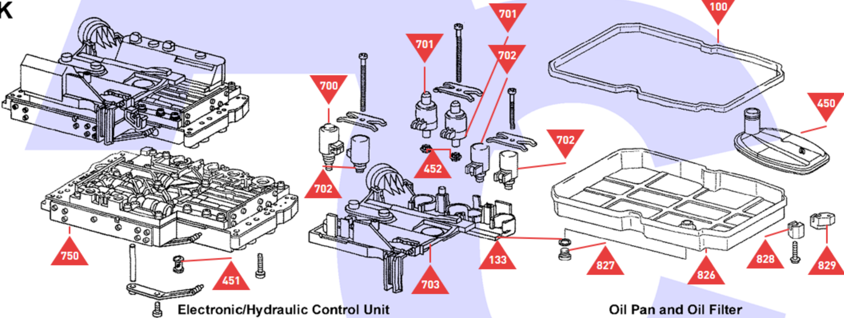
Electronic/Hydraulic Control Unit
