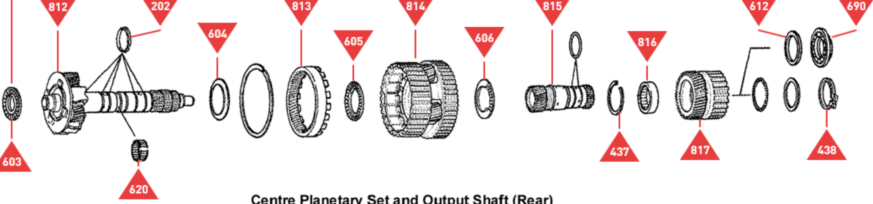
Centre Planetary Set and Output Shaft (Rear)
