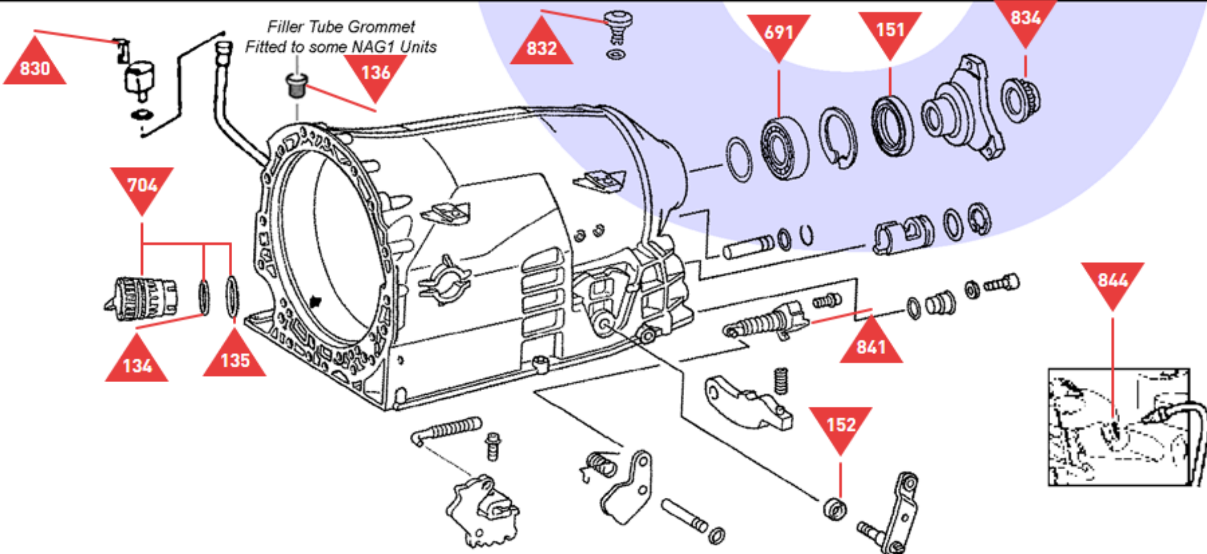
Transmission Housing, Output Flange and Ancillary Parts
