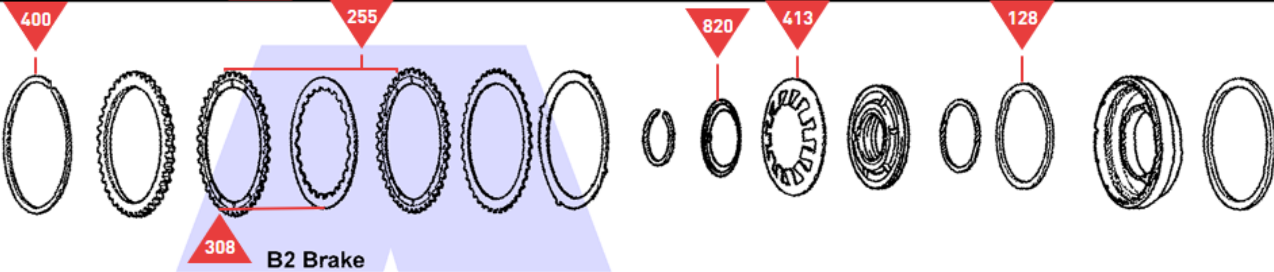
B2 Brake
