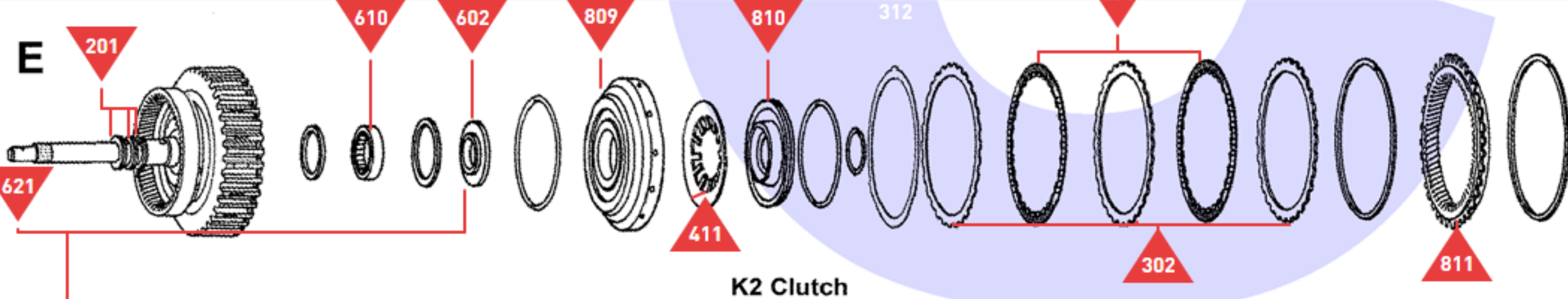
K2 Clutch
