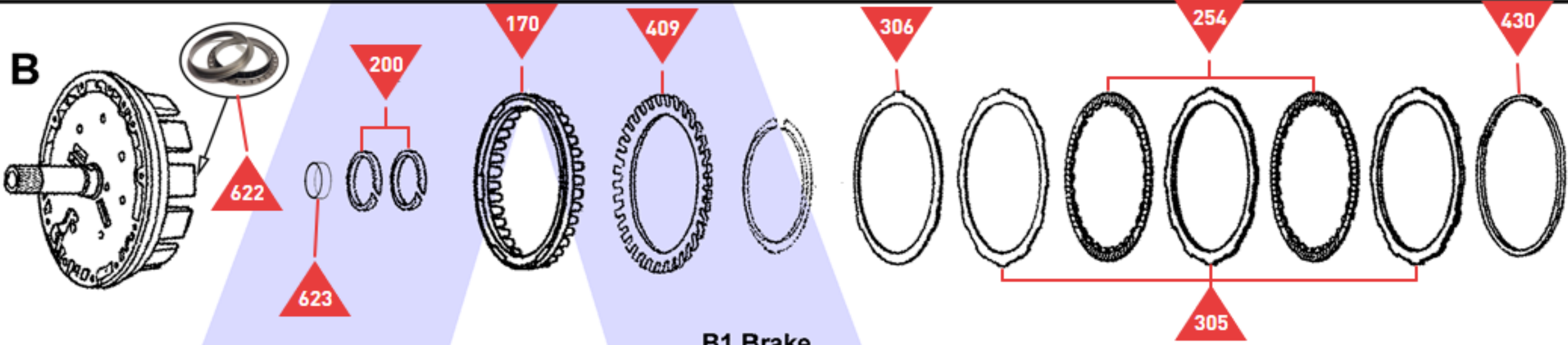
B1 Brake
