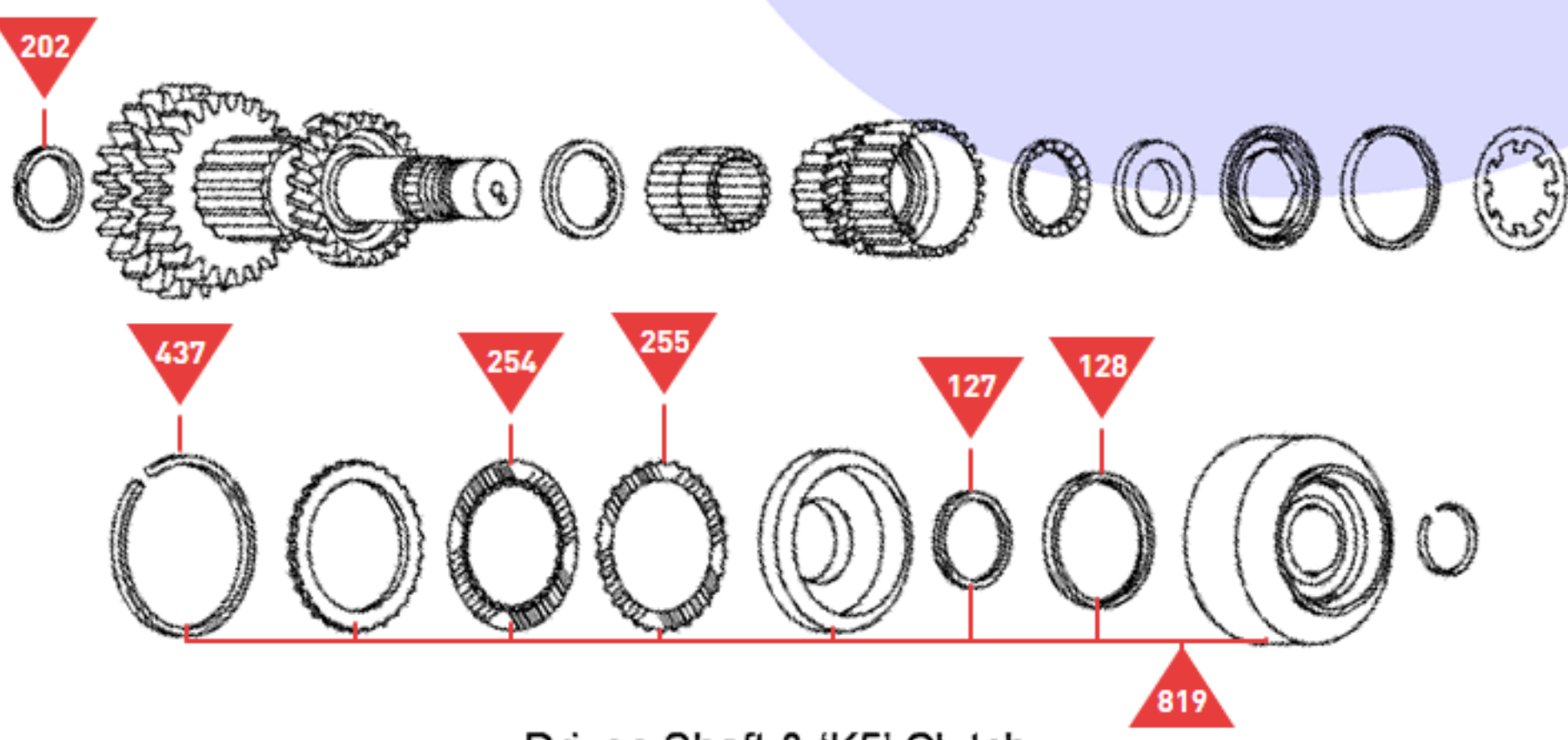
Driven Shaft & 'K5' Clutch
