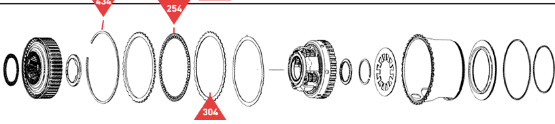
'B06' Brake and Planetary Gearset No. 3
