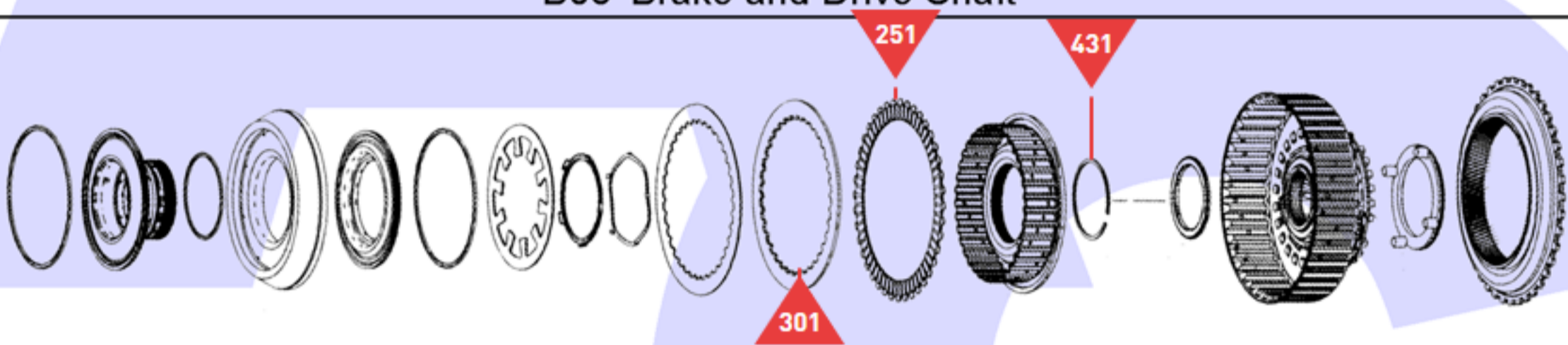
'K81' Clutch and Planetary Gearset No. 1
