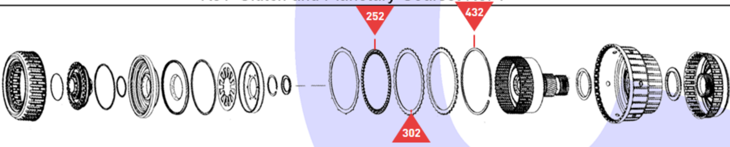
'K38' Clutch and Planetary Gearset No. 2
