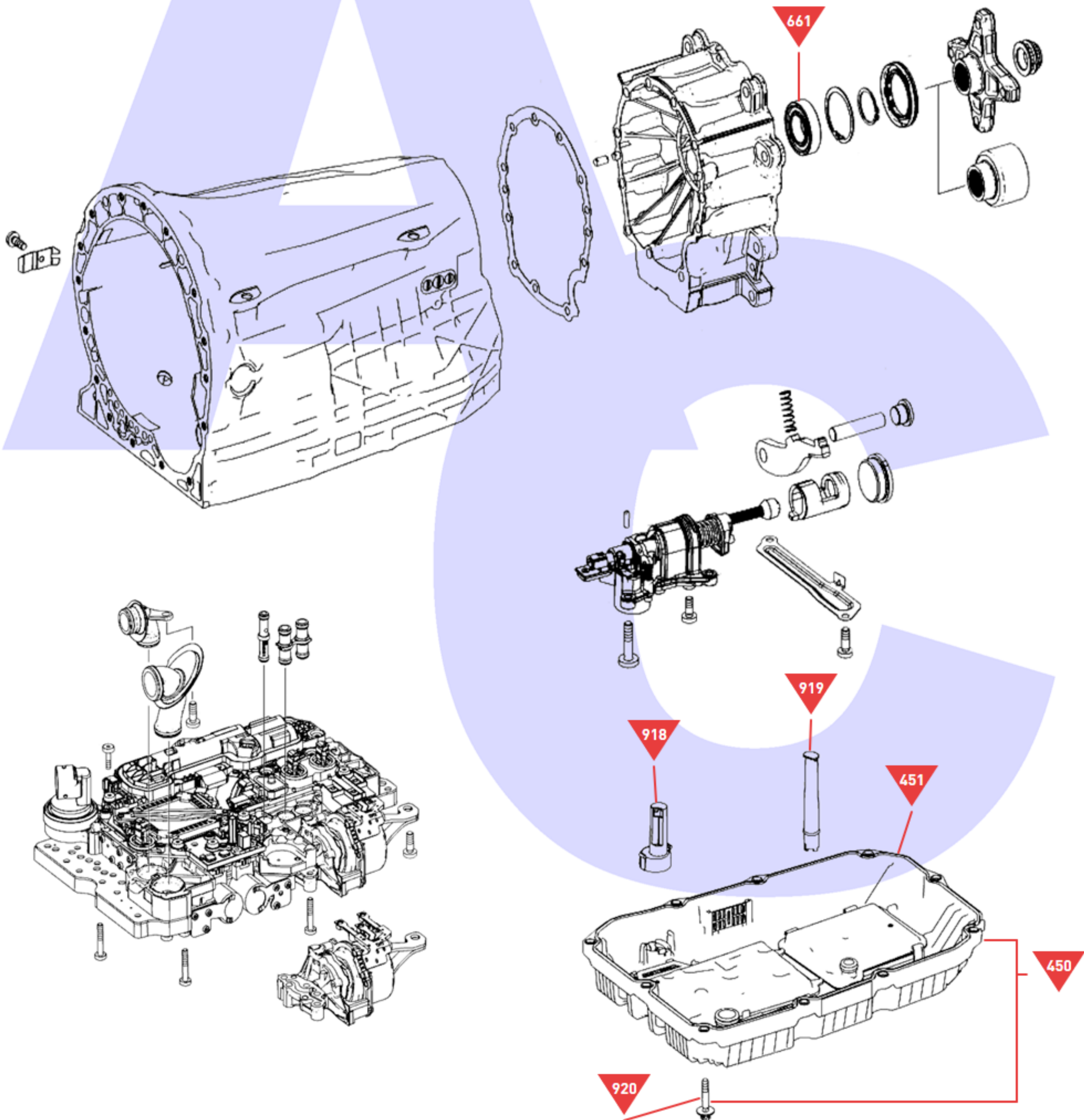
Casing, Output, Mechatronic, External Components, Internal Components, Oil Pan and Filters
