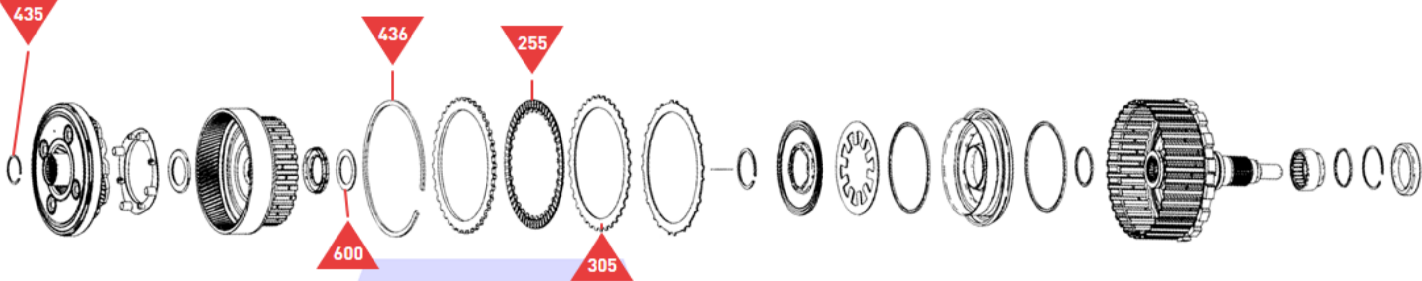
'K27' Clutch and Planetary Gearset No. 4
