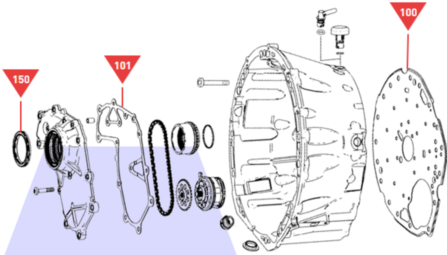
Converter Housing and Oil Pump
