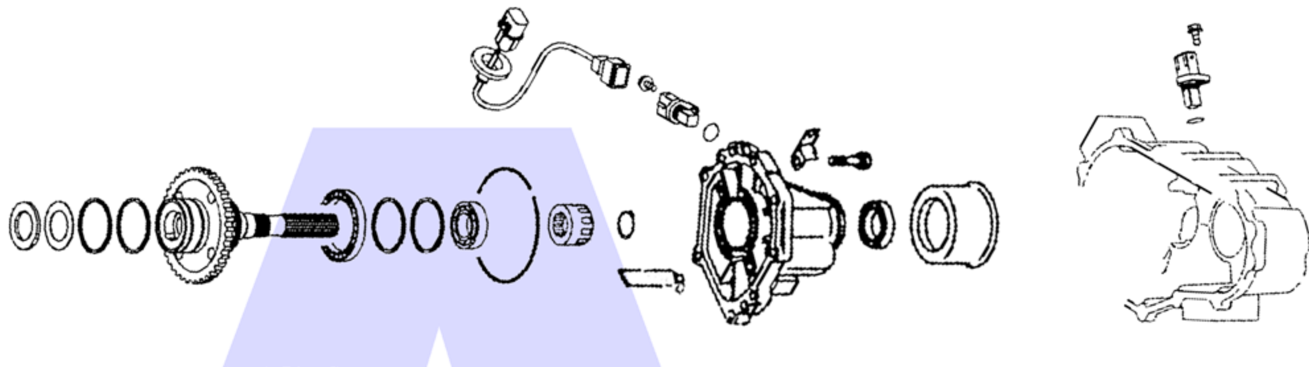
Output Shaft
