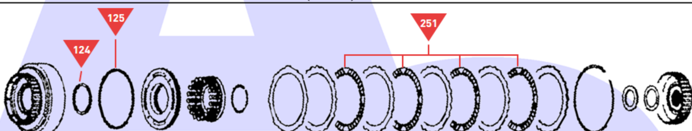
Front (Direct) Clutch
