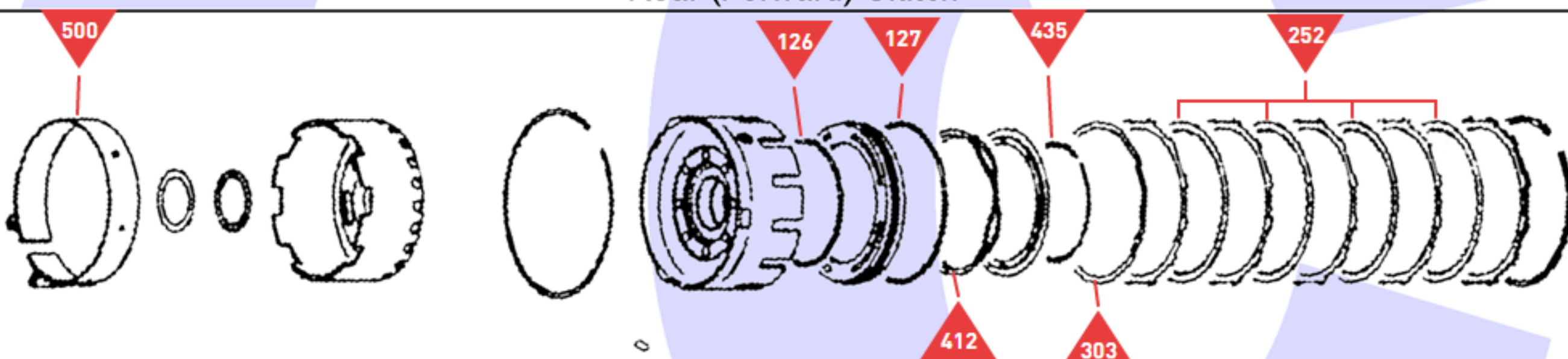
2-4 Band and Low Reverse Brake
