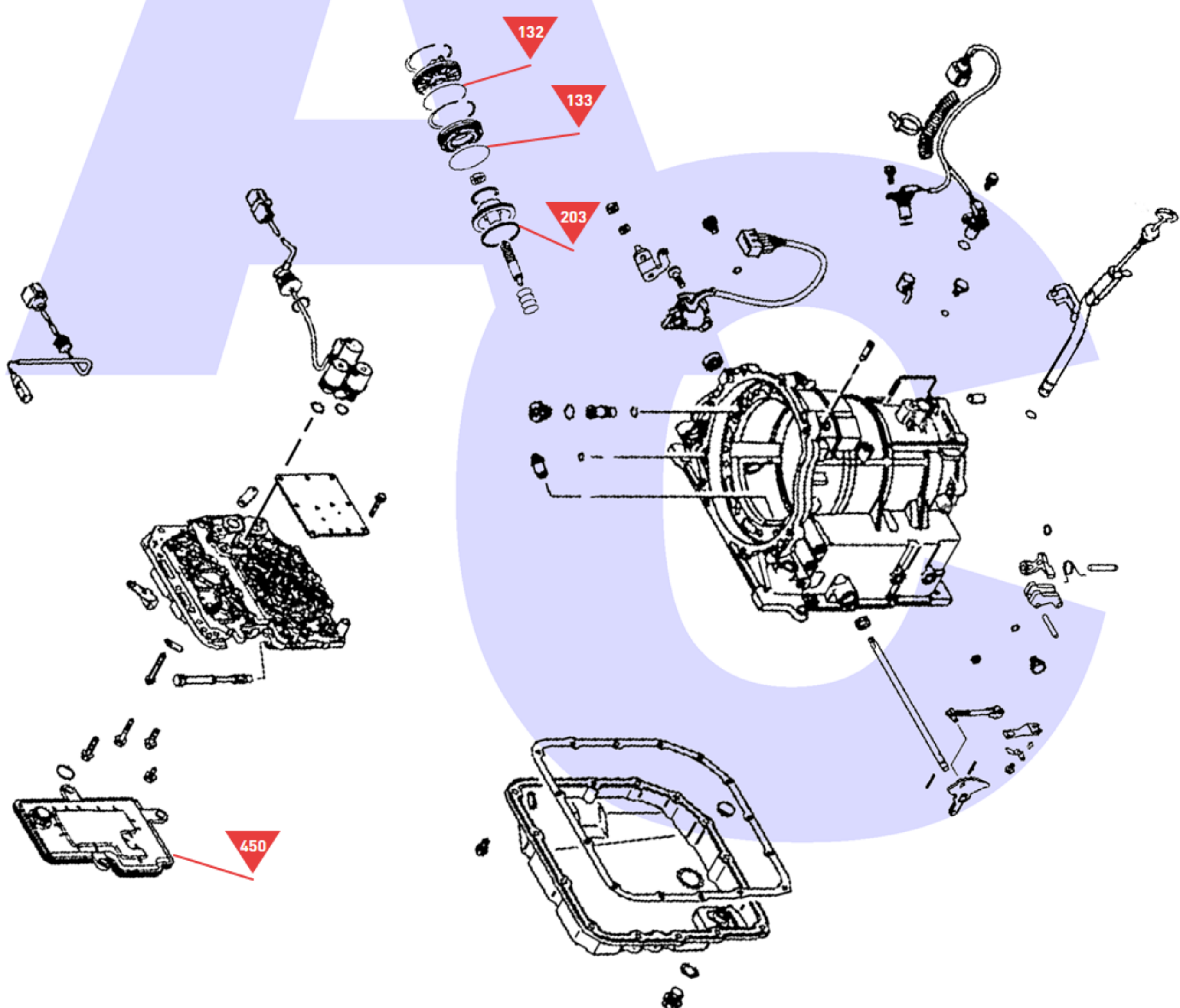
Main Case, 2-4 Servo, Valve Body and Associated Components
