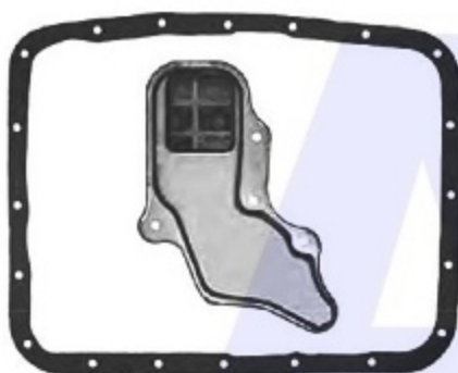
4EAT Legacy & SVX Pan Gasket SUB4.GAS01 Filter SUB4.FIL01 No Pick Up Spout 1987-1998
