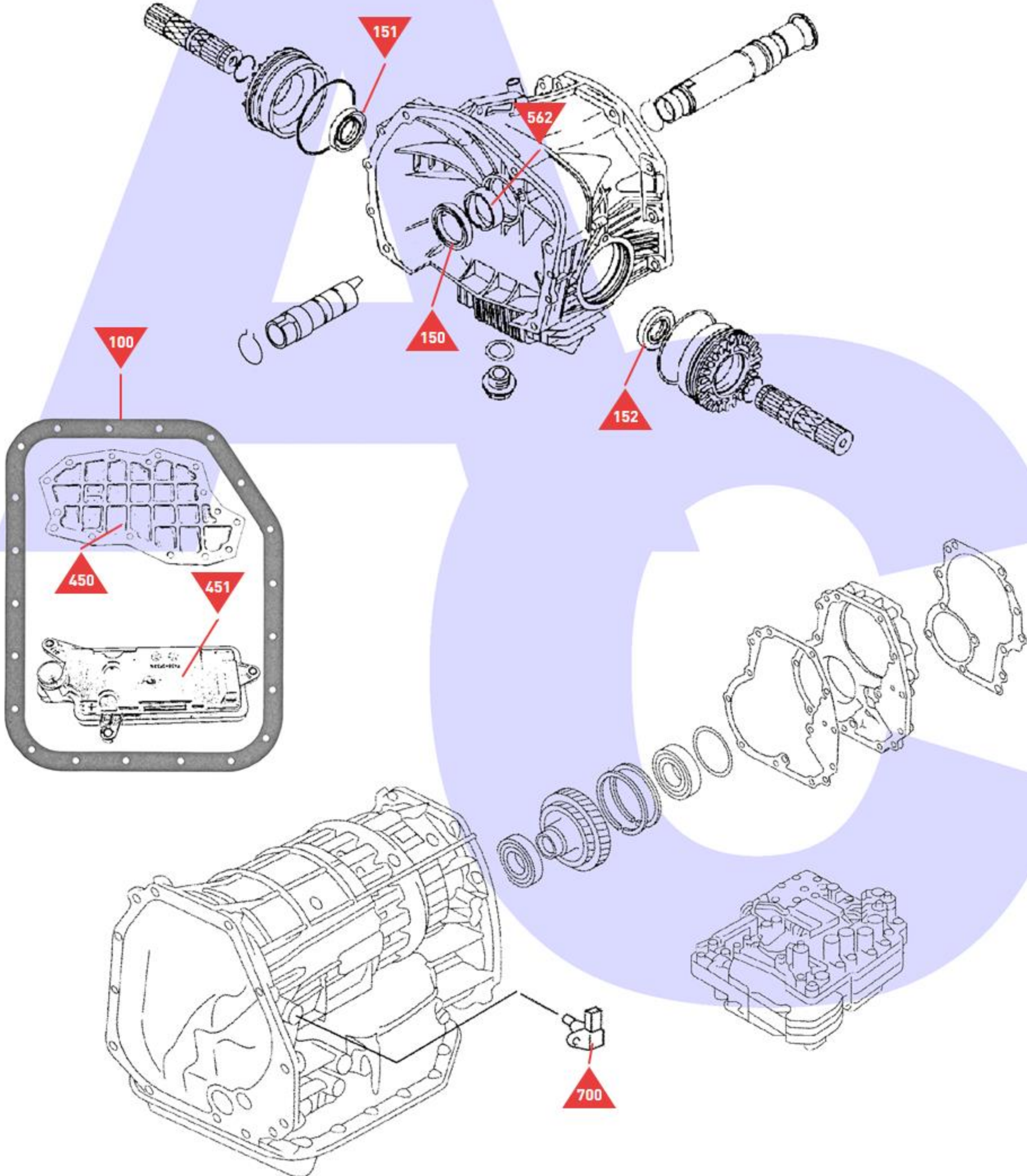
Case, Valve Body Components & Reduction Drive Gear
