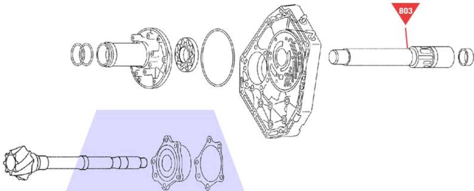
Oil Pump & Pinion Shaft
