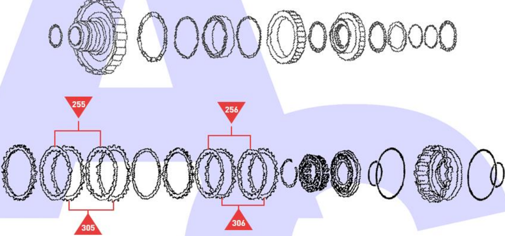
Forward Brake & Low Coast Brake
