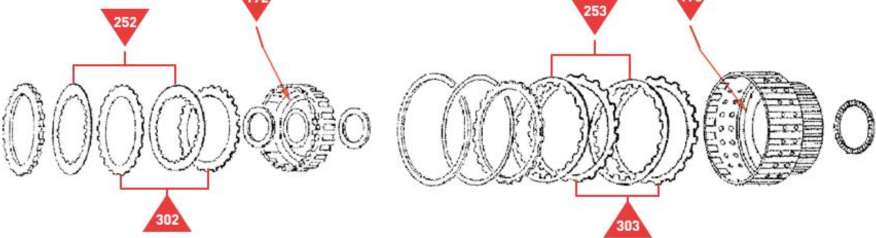
High & Low Reverse Clutch
