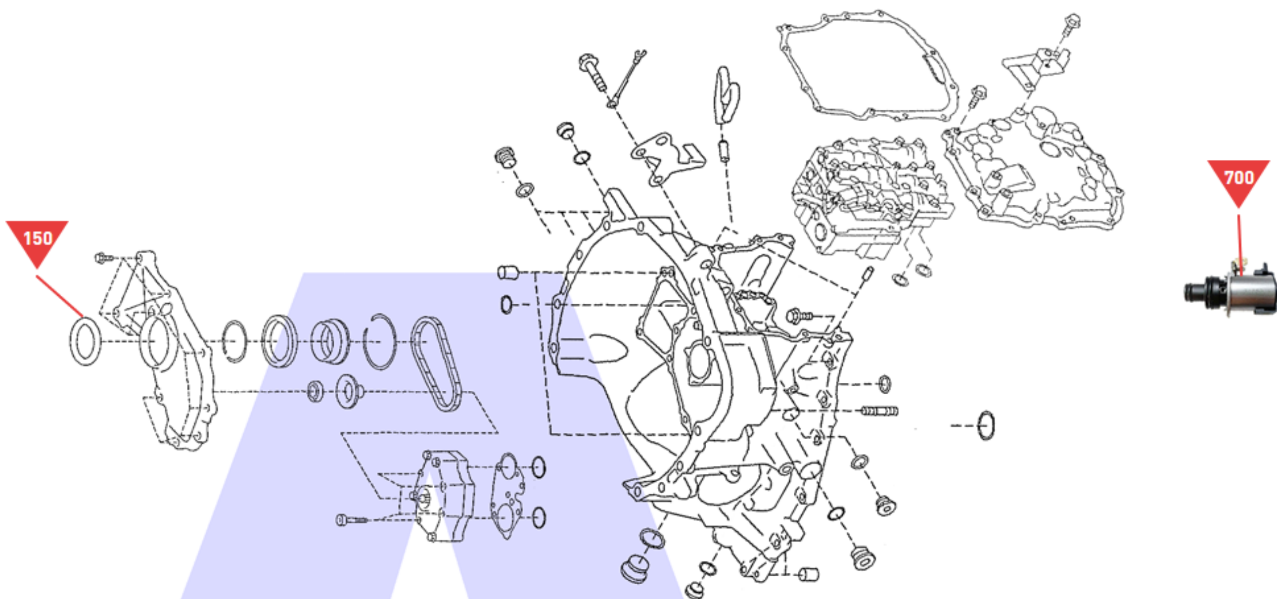
Oil Pump, Bell Housing, Valve Body and External Components
