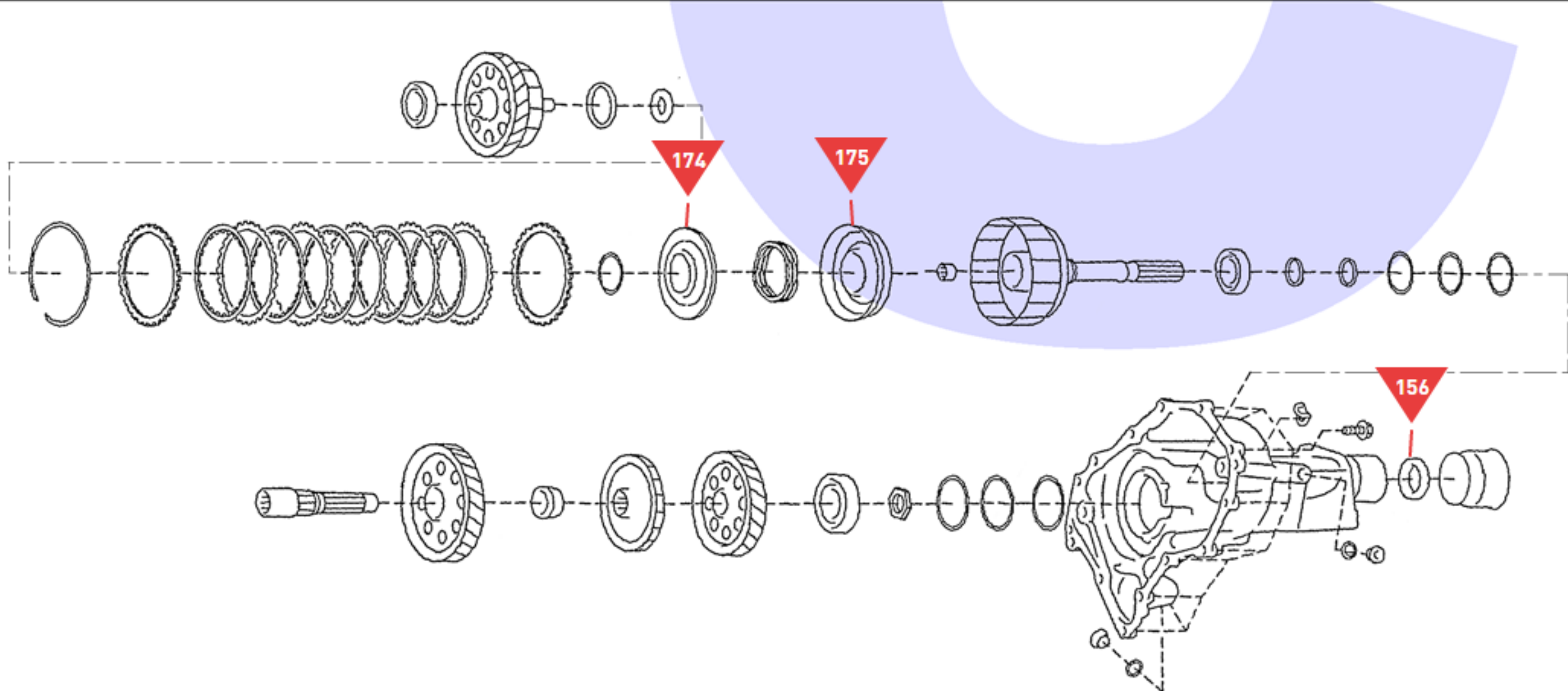
Transfer Gear, Transfer Clutch, Output Clutch and Extension Housing
