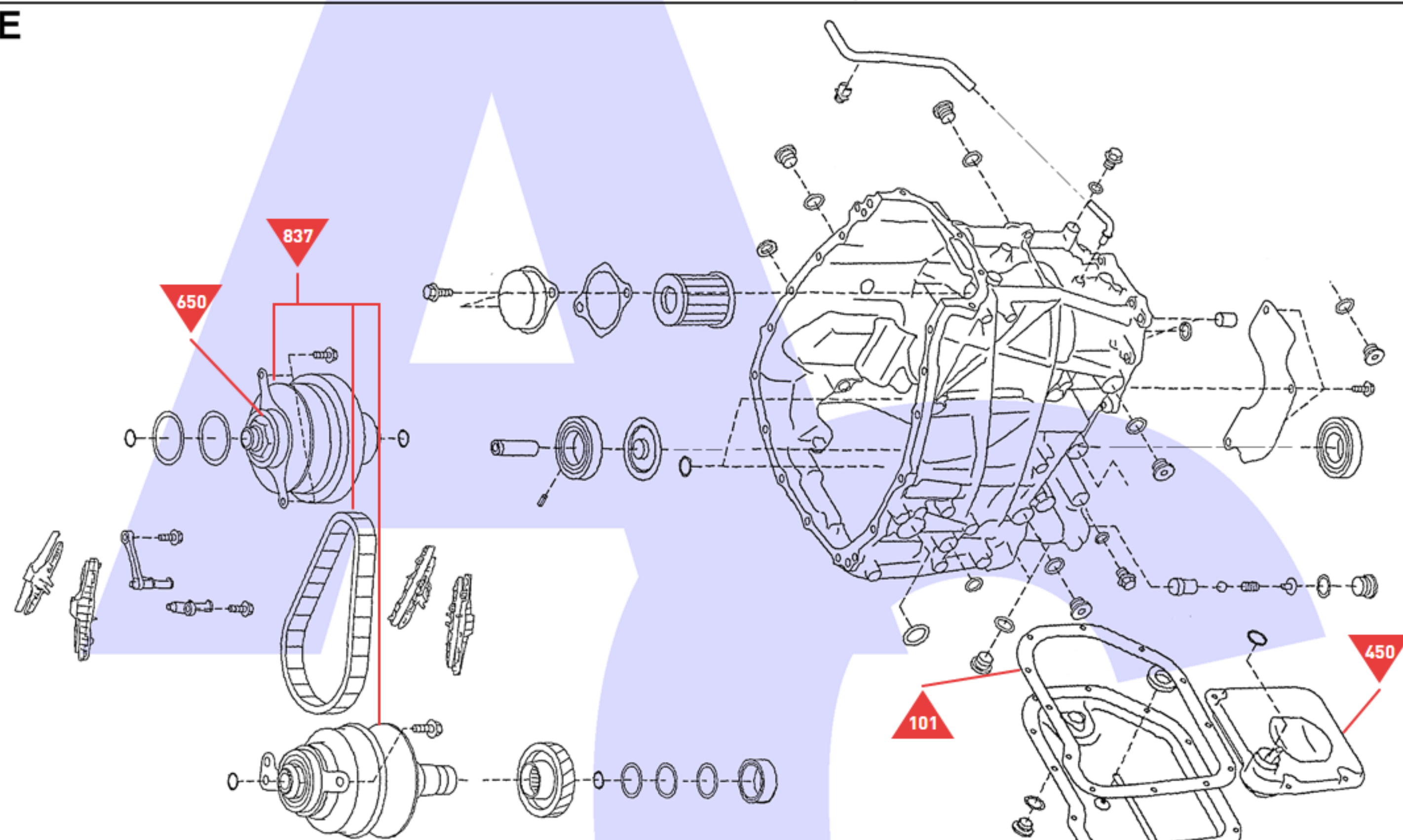
Primary Pulley, Secondary Pulley, Drive Chain, Main Case Etc.
