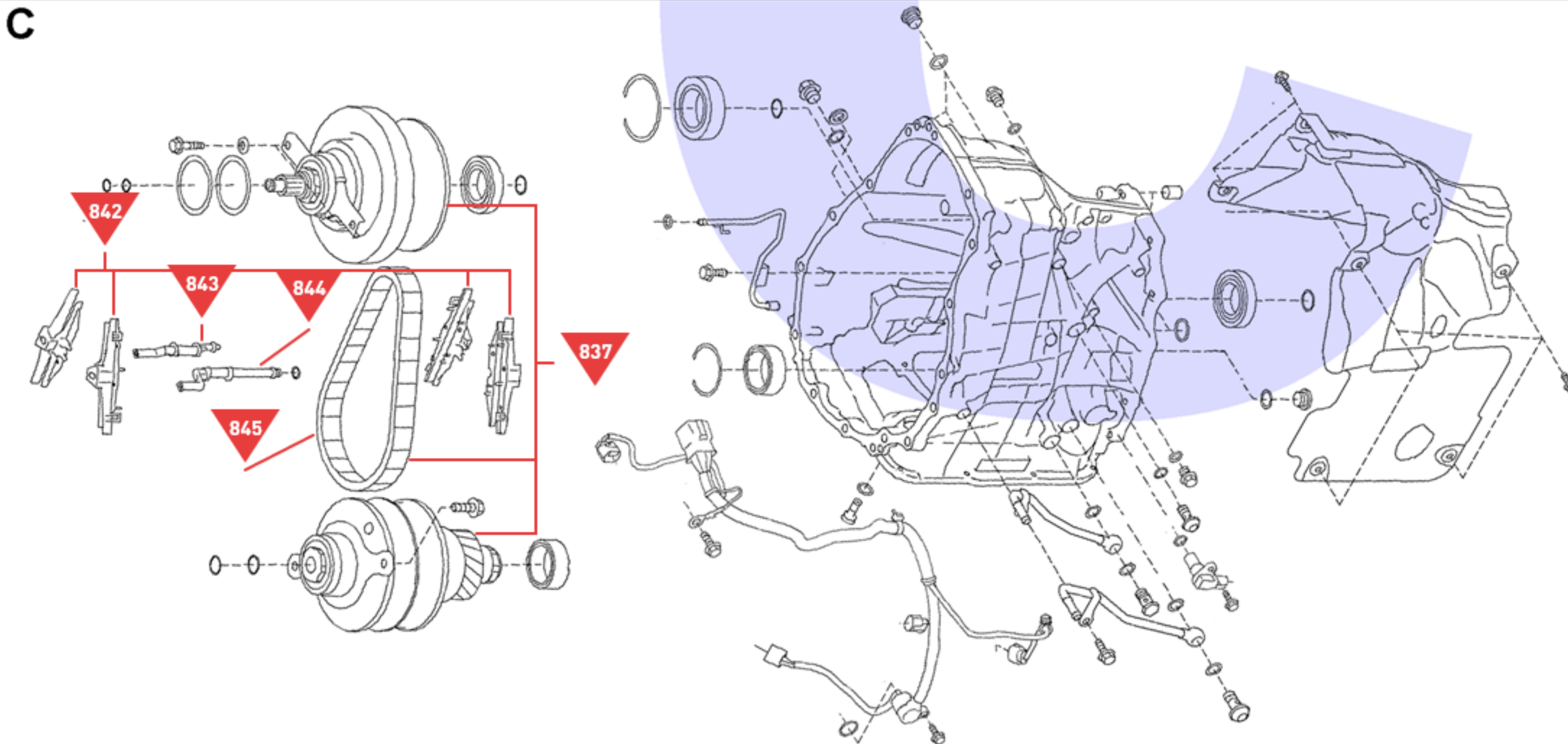
Pulley Set and Main Case
