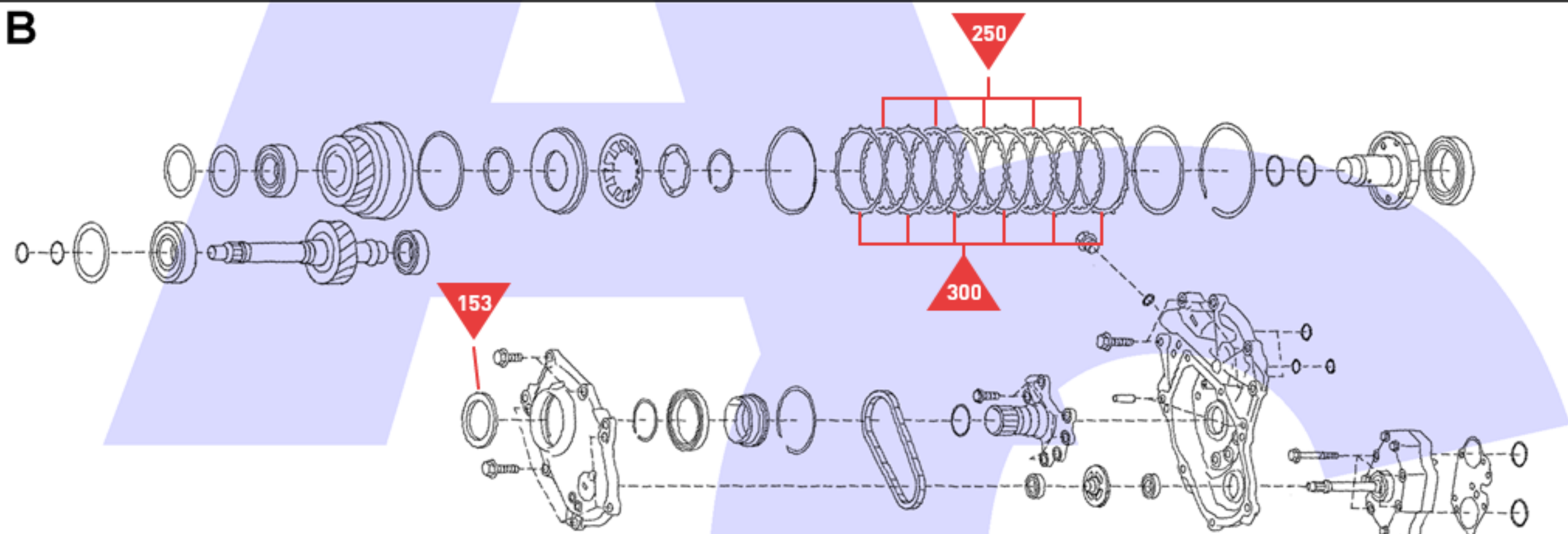
Bell Housing and Front Differential
