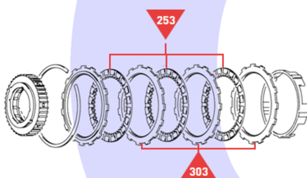
One Way Clutch No. 1 and 2nd Brake
