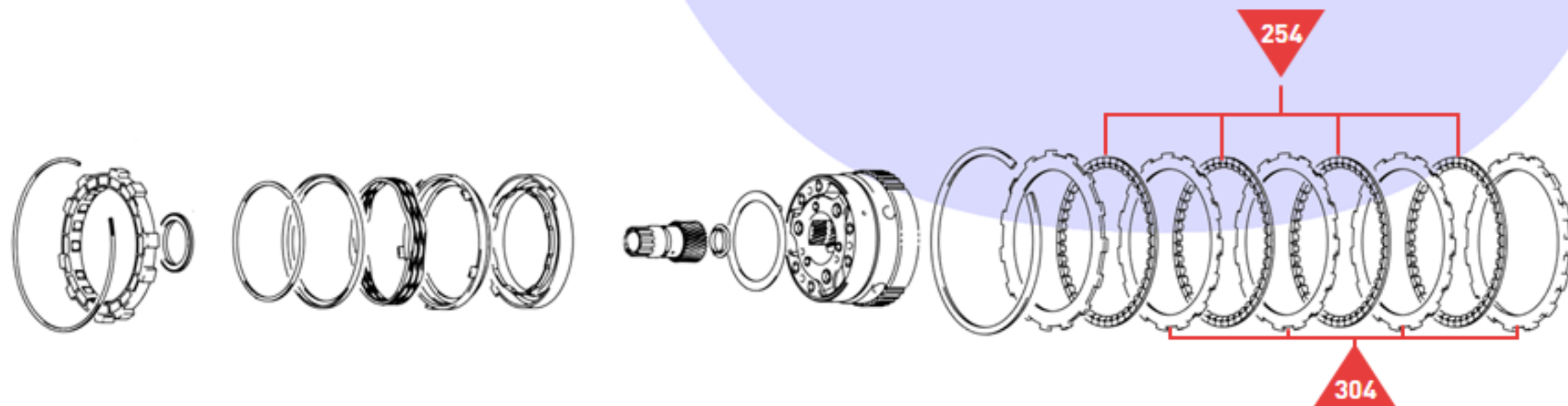
One Way Clutch No.2, 2nd Brake Piston, Rear Sun Gear, Planetary, 1st and Reverse Brake
