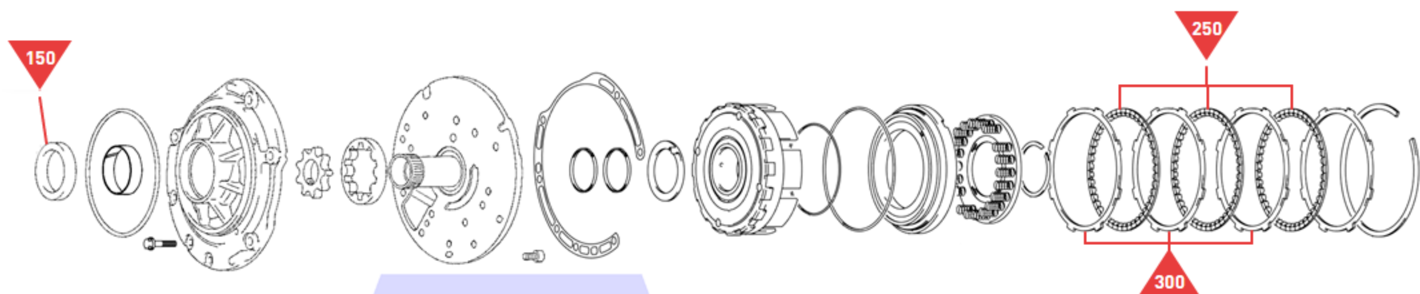
Oil Pump and Reverse Clutch
