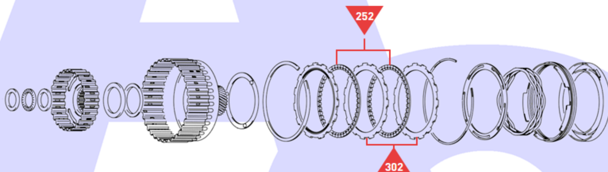
Forward Hub, Front Sun Gear, Overdrive and 2nd Coast Brake
