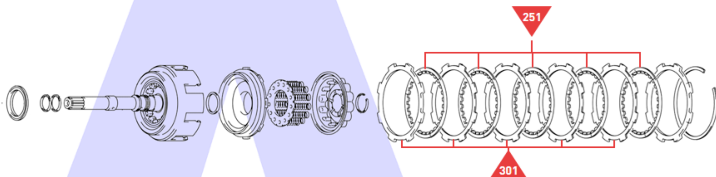
Forward Clutch and Input Shaft
