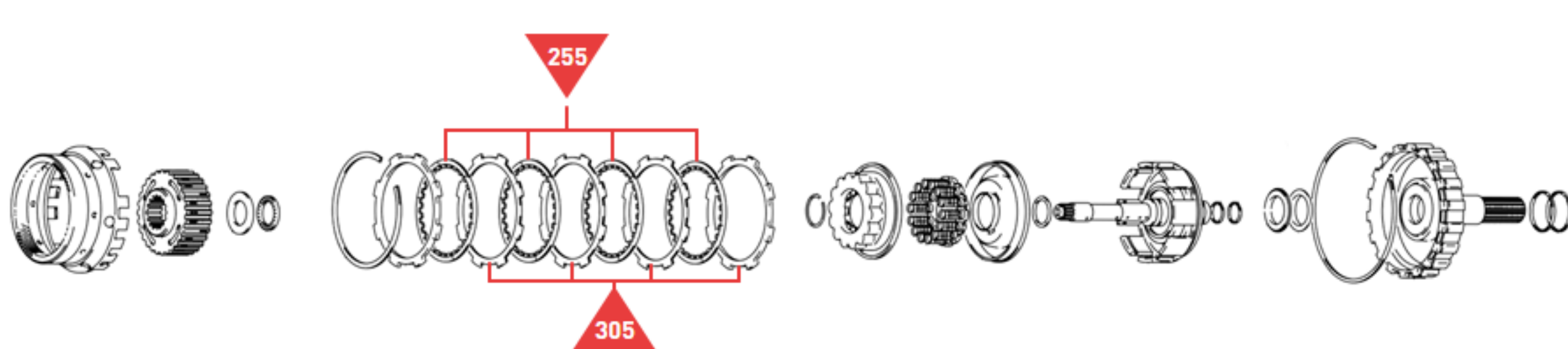
Ring Gear, Direct Clutch and Output Shaft
