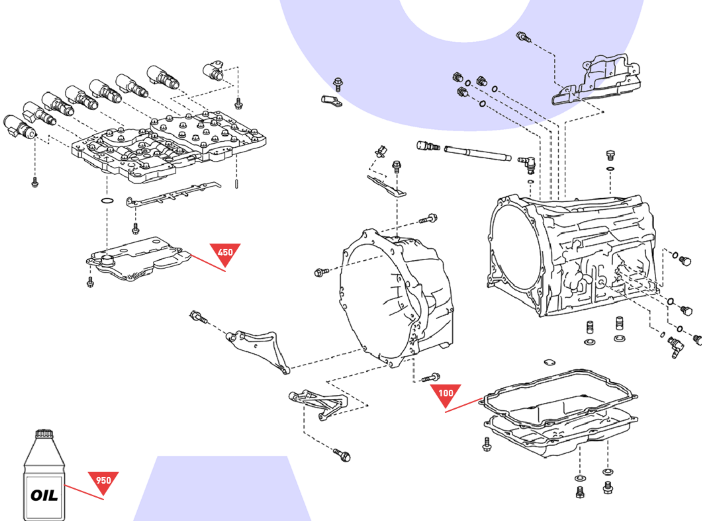
Valve Body, Oil Strainer, Transmission Case & Oil Pan
