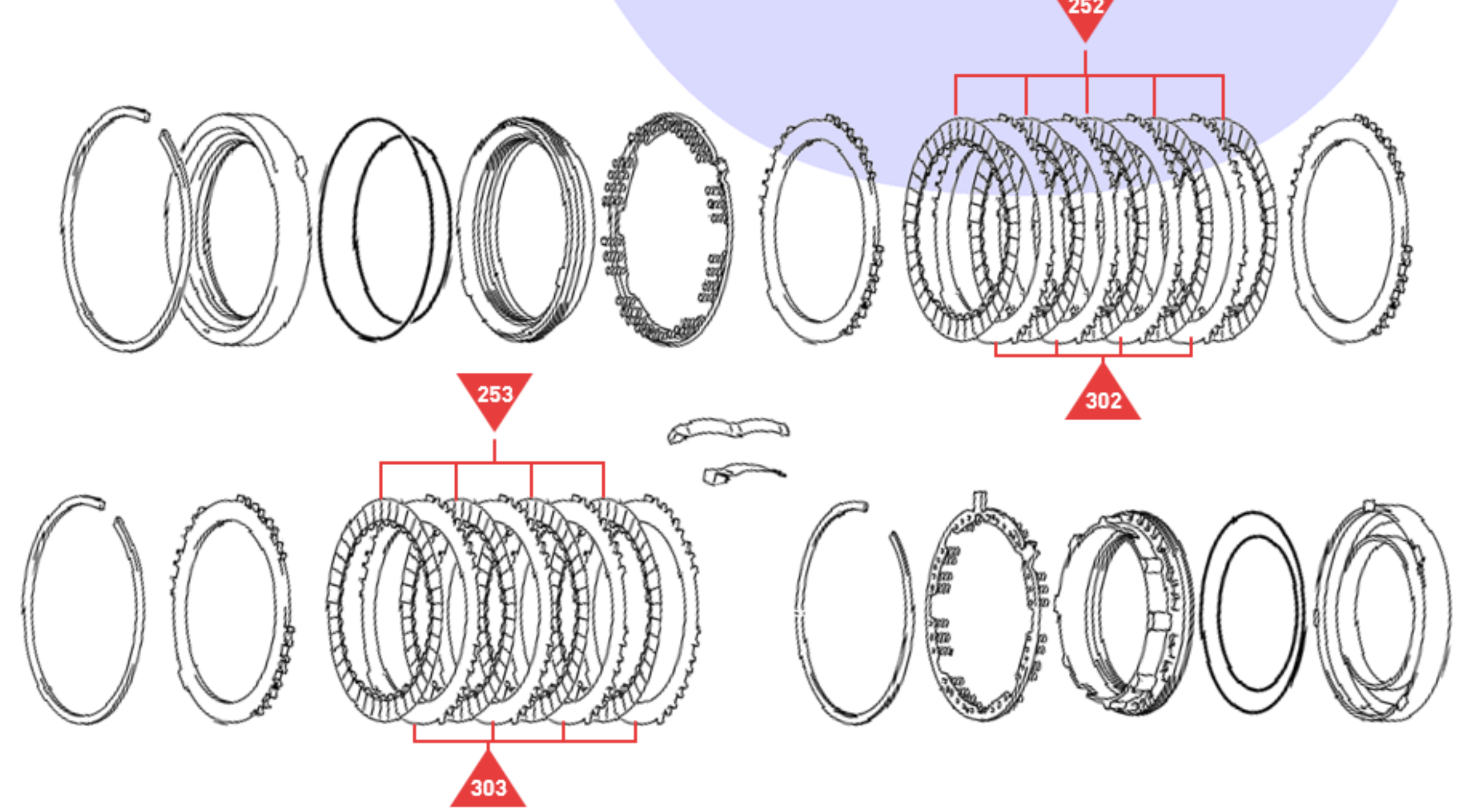
Brake No. 2 & Brake No. 1
