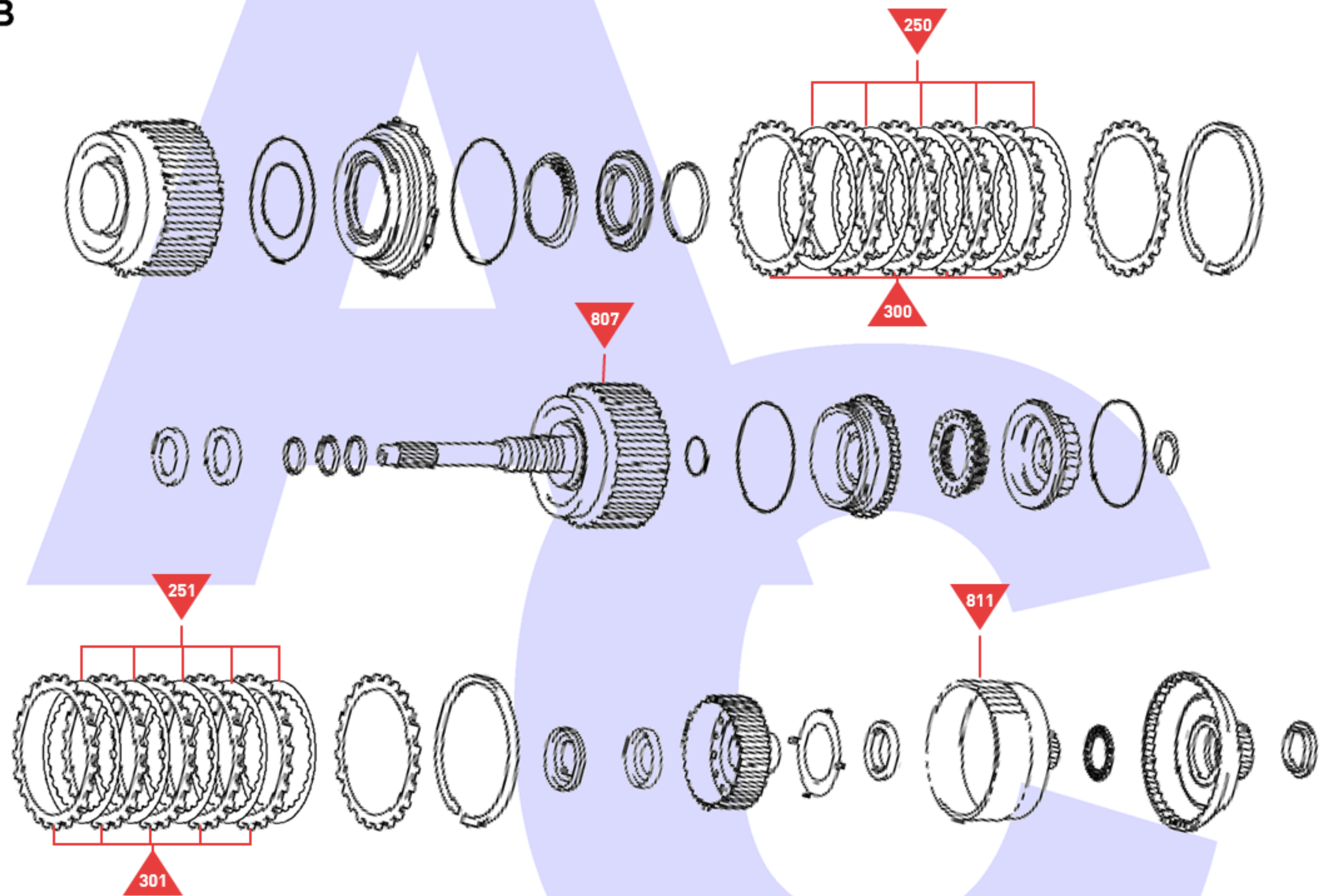
Brake Band, Direct Clutch & Forward Clutch
