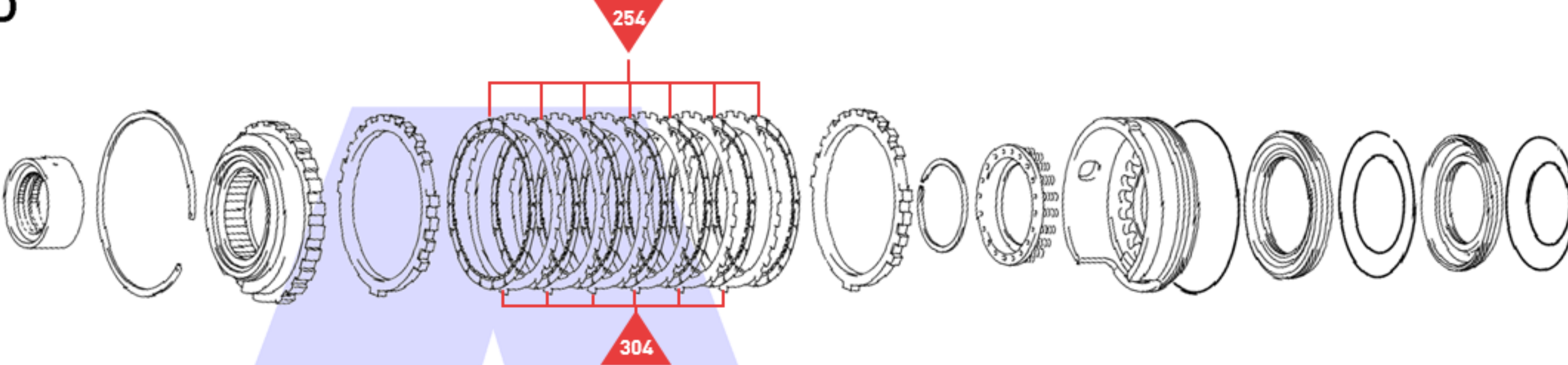
Brake No. 3, 1st & Reverse Brake
