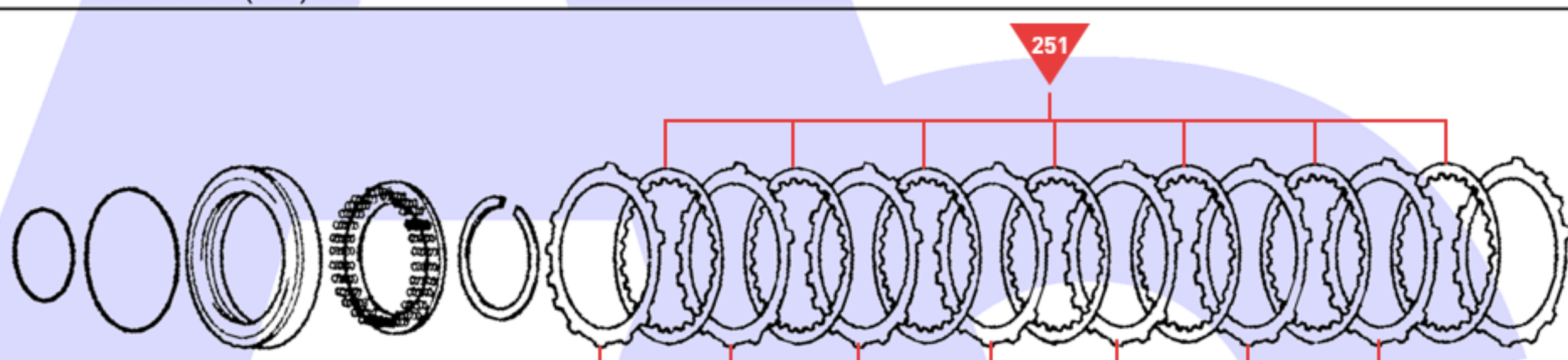
Forward (C1) Clutch
