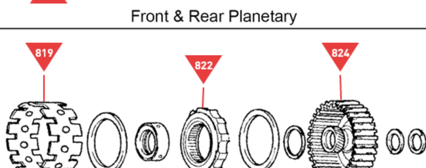
Front & Rear Planetary
