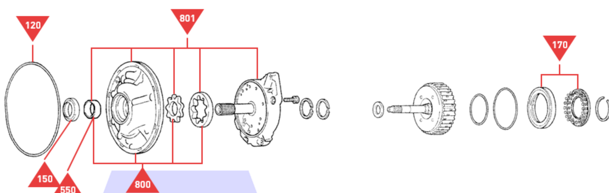
Oil Pump & Forward (C1) Clutch Drum
