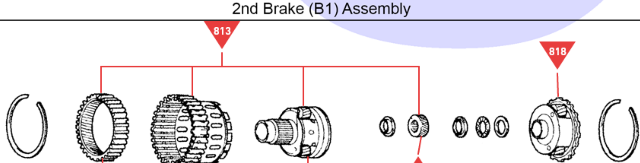
2nd Brake (B1) Assembly
