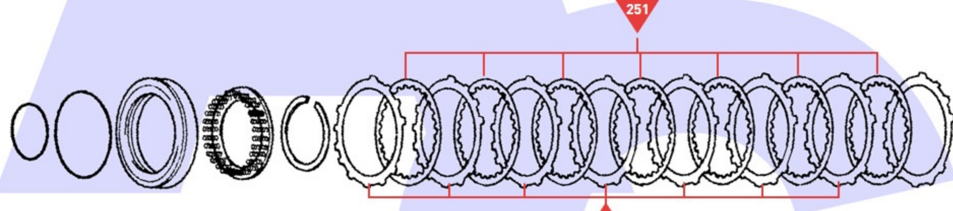
1st & Reverse Brake (B2) Assembly
