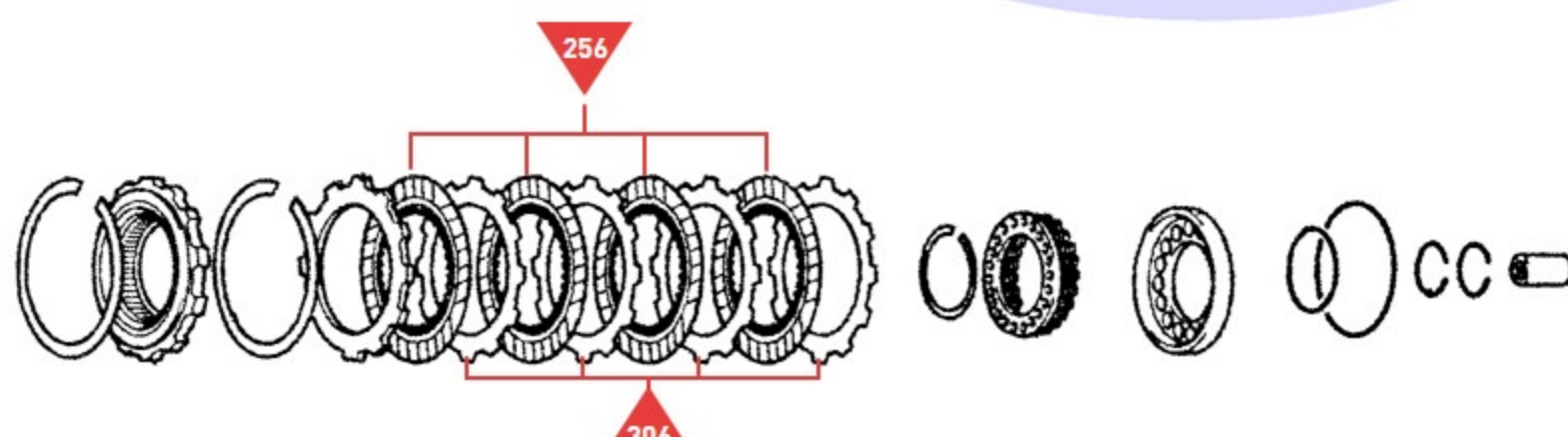
No. 2 One-Way-Clutch (F2) & Underdrive Brake (B3) Assembly
