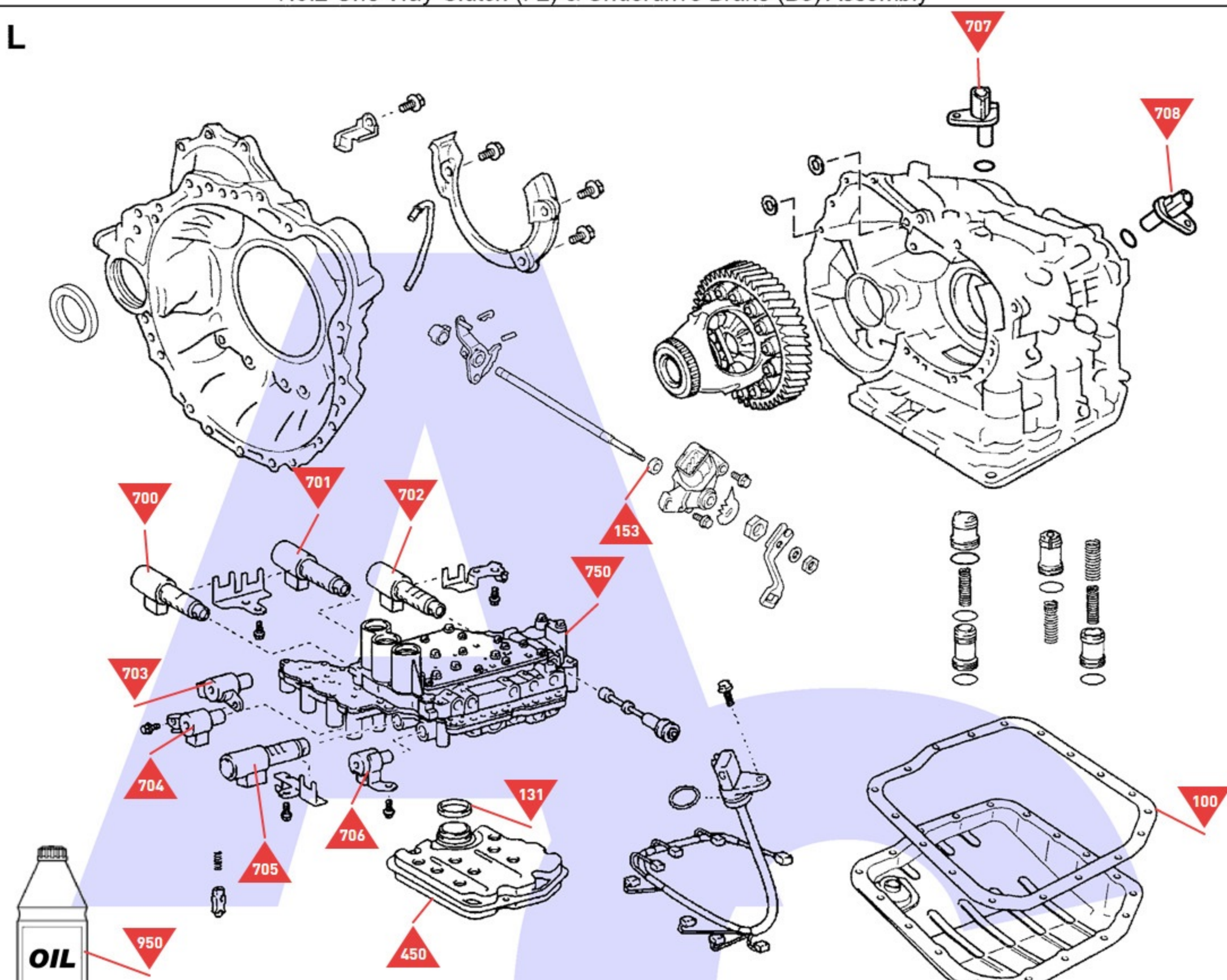
Maincase, Differential, Valve Body & Related Components
