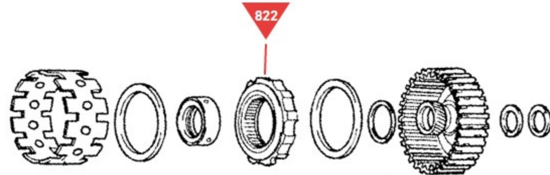
No. 1 One-Way-Clutch (F1) Assembly & Rear Planetary Sun Gear
