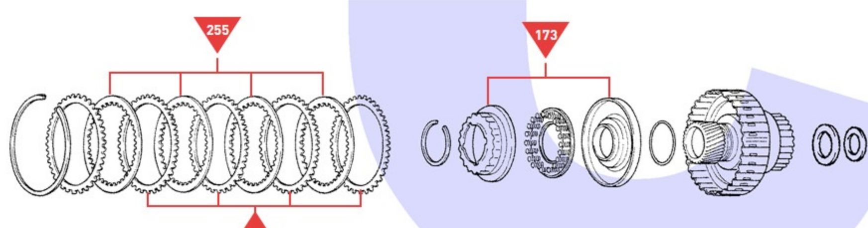
Underdrive Clutch (C3) Assembly
