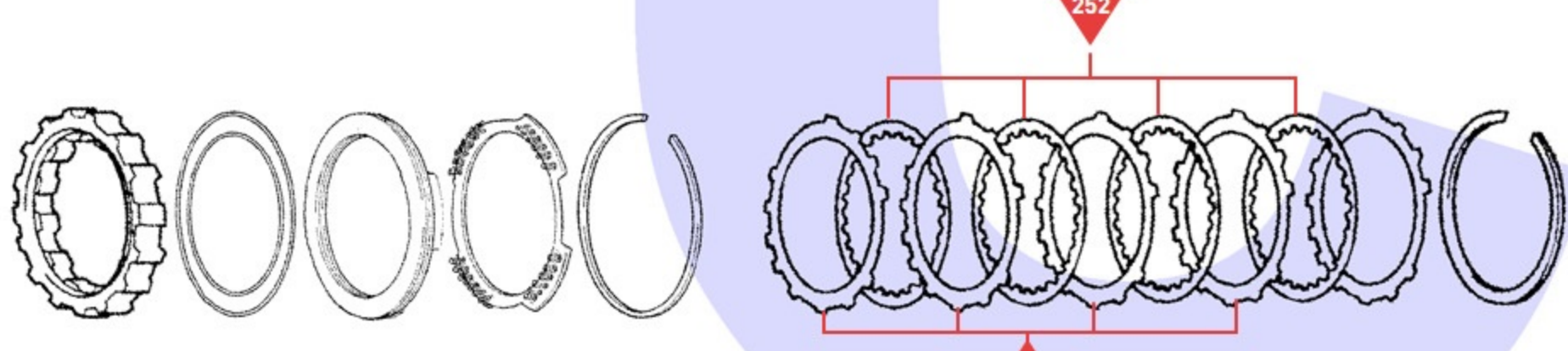
2nd Brake (B1) Assembly
