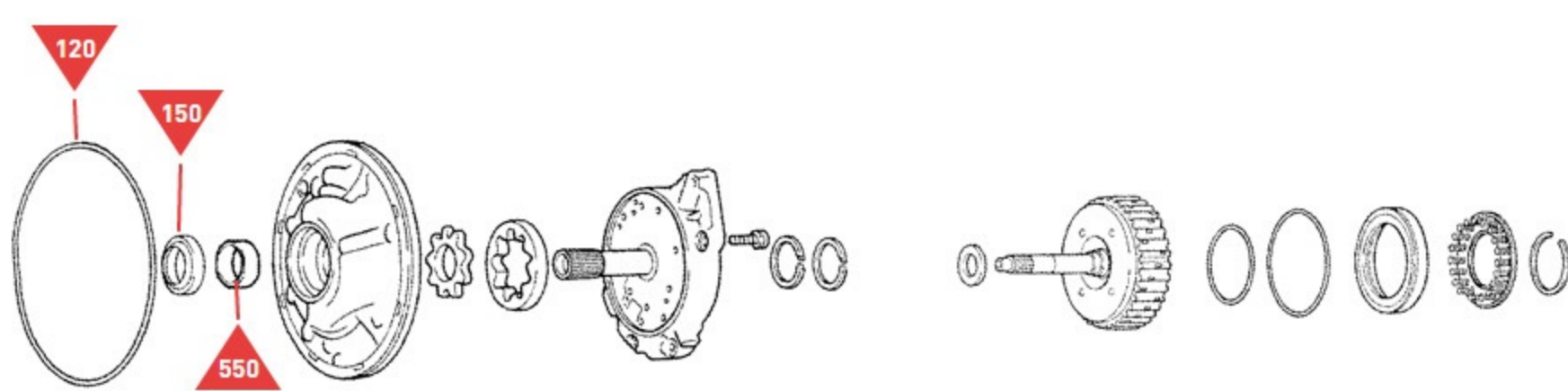
Oil Pump & Forward (C1) Clutch Drum
