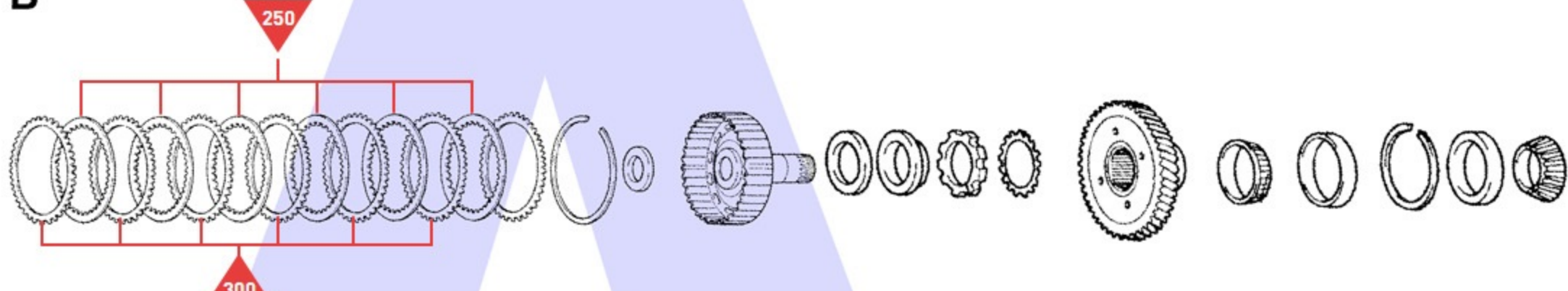
Forward (C1) Clutch
