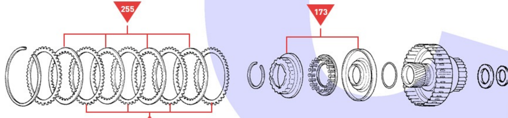
Underdrive Clutch (C3) Assembly
