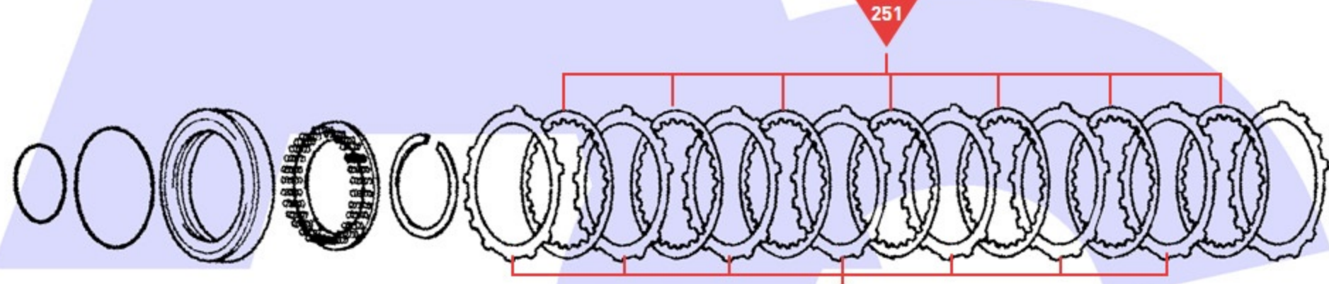
1st & Reverse Brake (B2) Assembly
