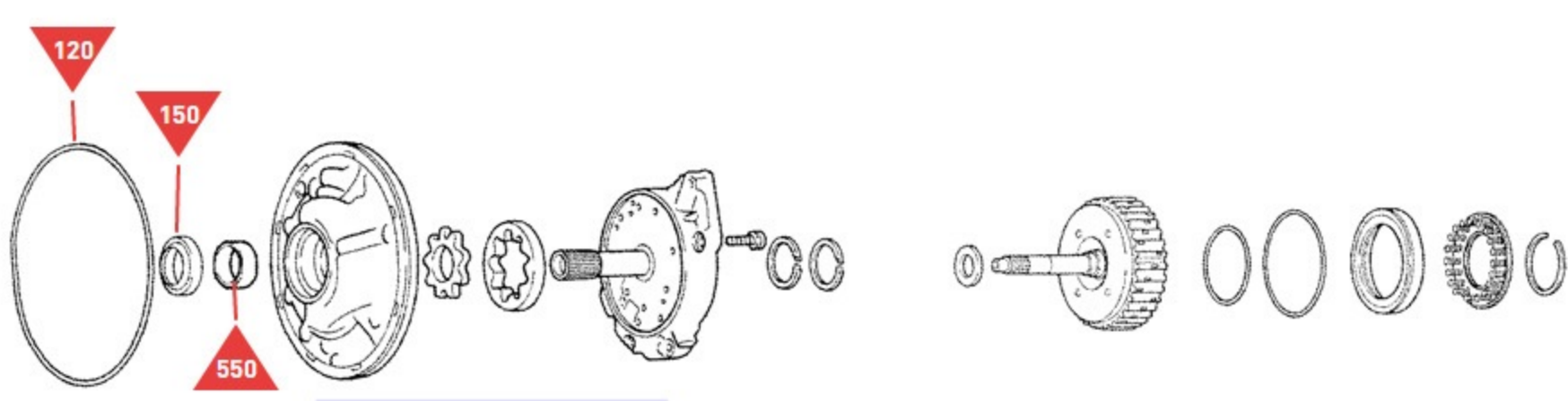
Oil Pump & Forward (C1) Clutch Drum
