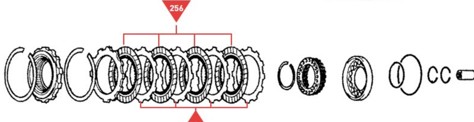
No.2 One-Way-Clutch (F2) & Underdrive Brake (B3) Assembly
