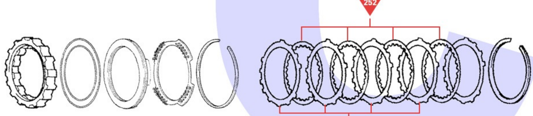
2nd Brake (B1) Assembly
