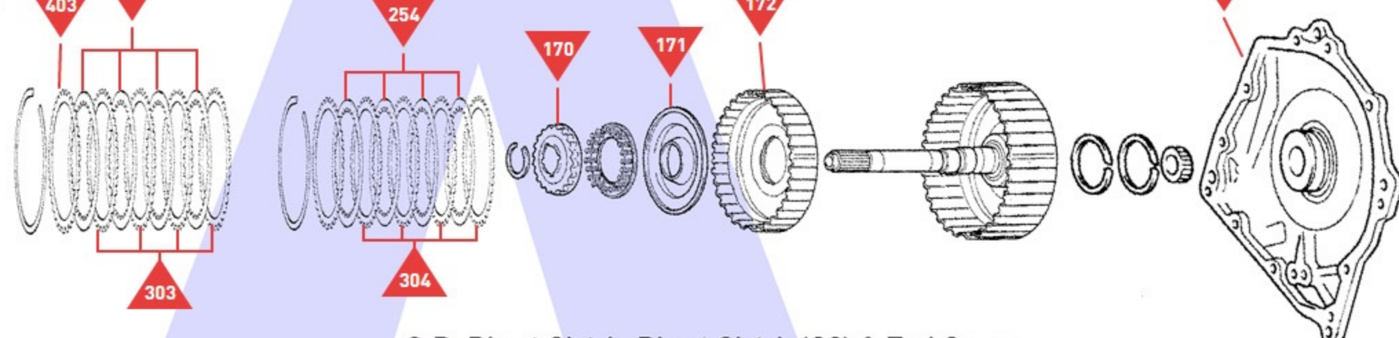
O.D. Direct Clutch, Direct Clutch (C2) & End Cover
