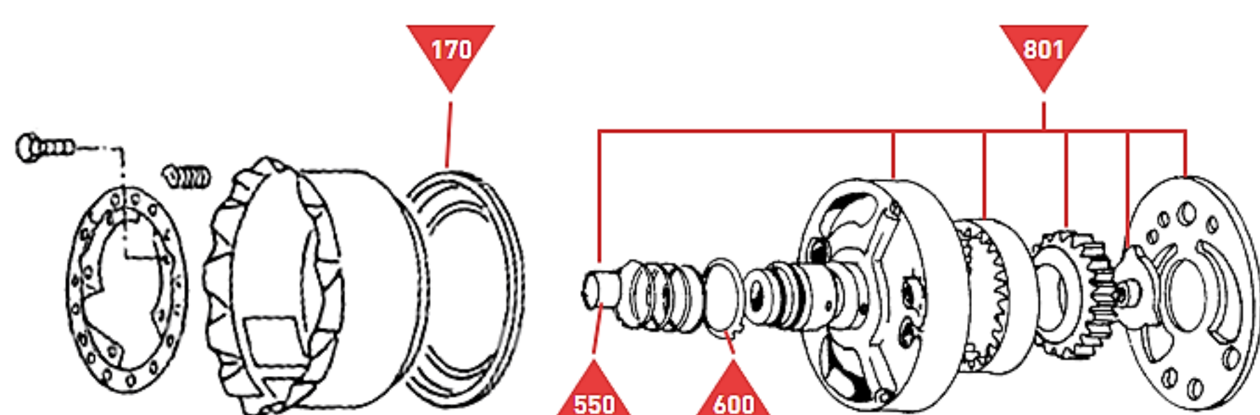
Oil Pump
