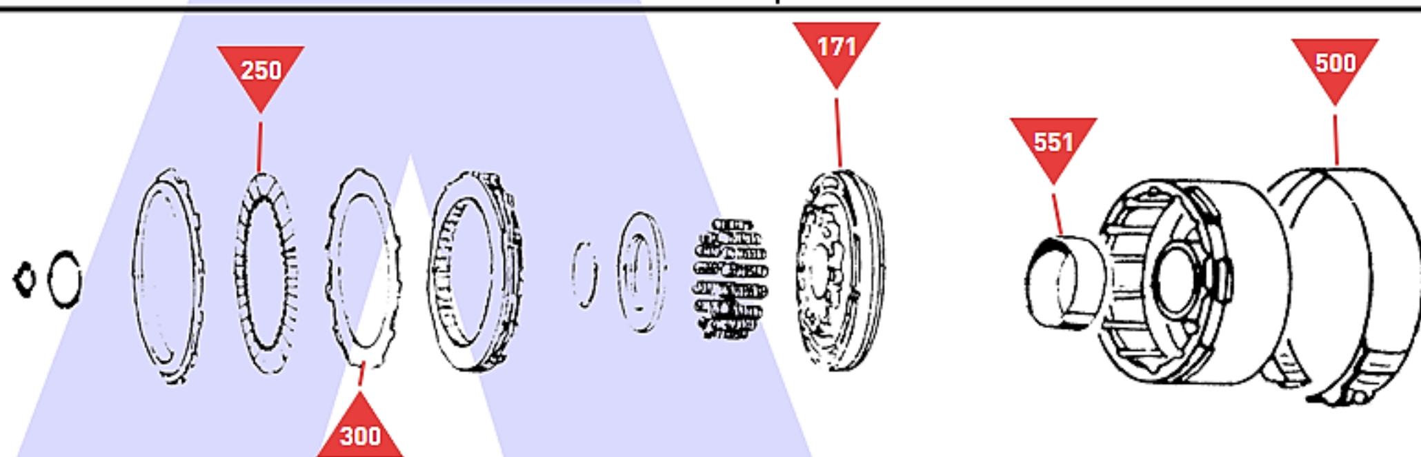
Direct Clutch
