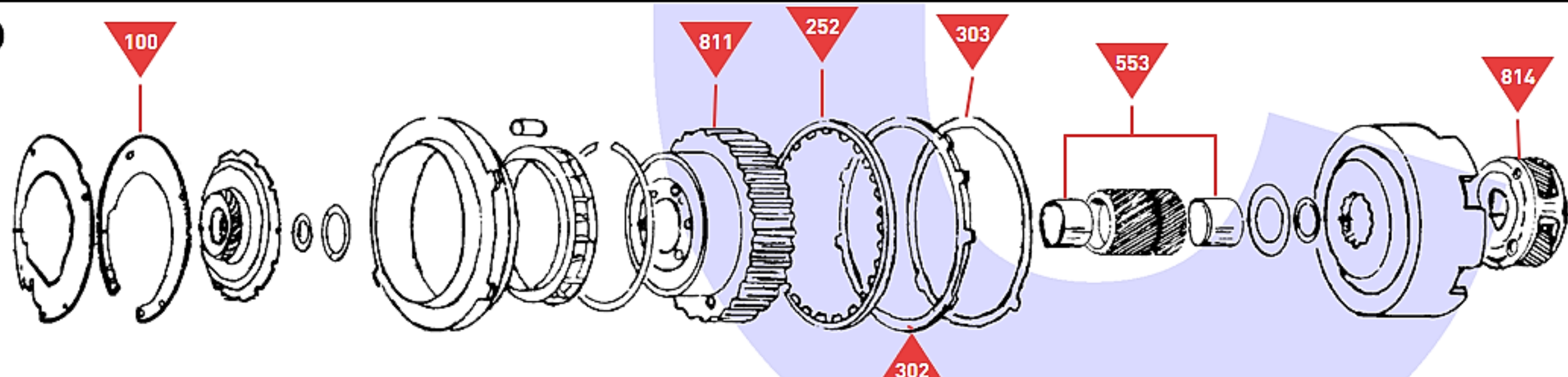
Planetary Sets and Low Reverse Brake
