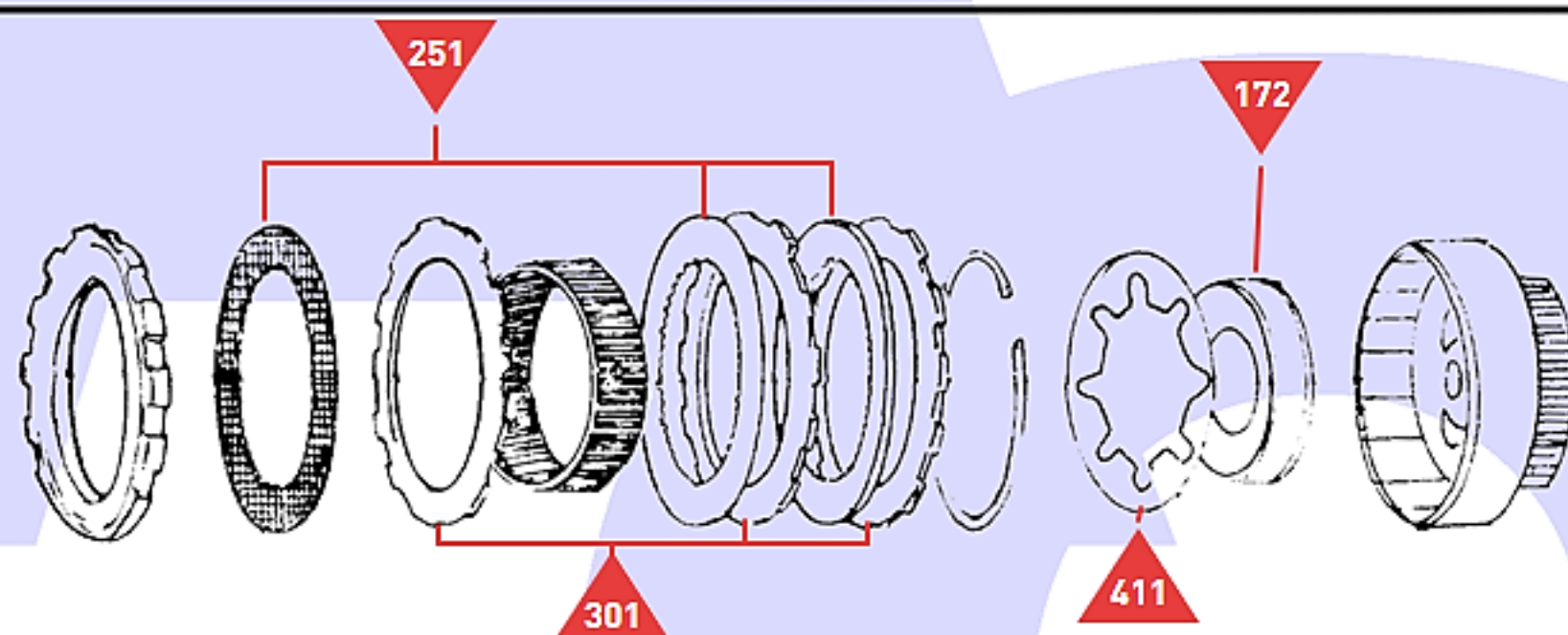
Forward Clutch
