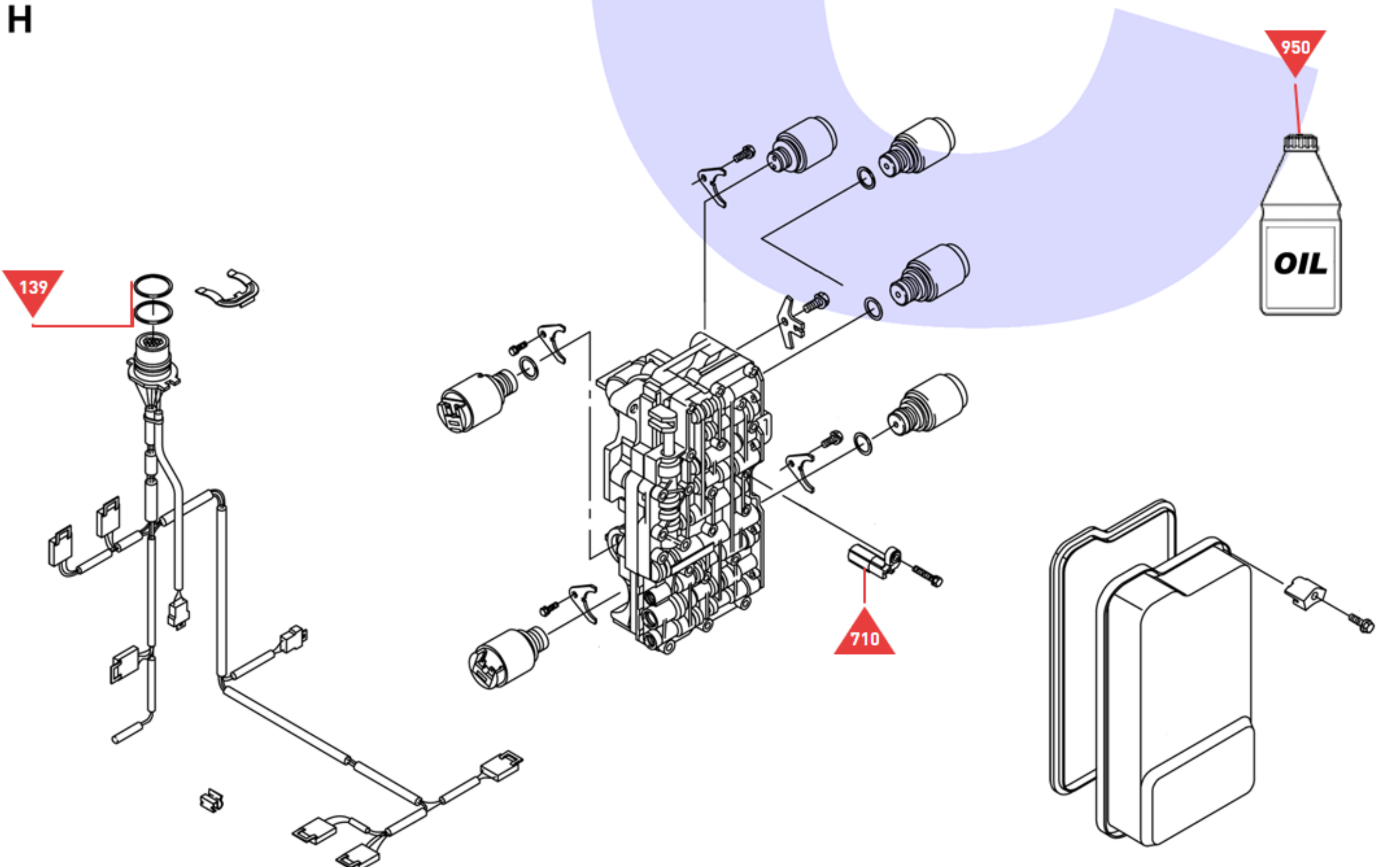
Valve Body and Associated Components
