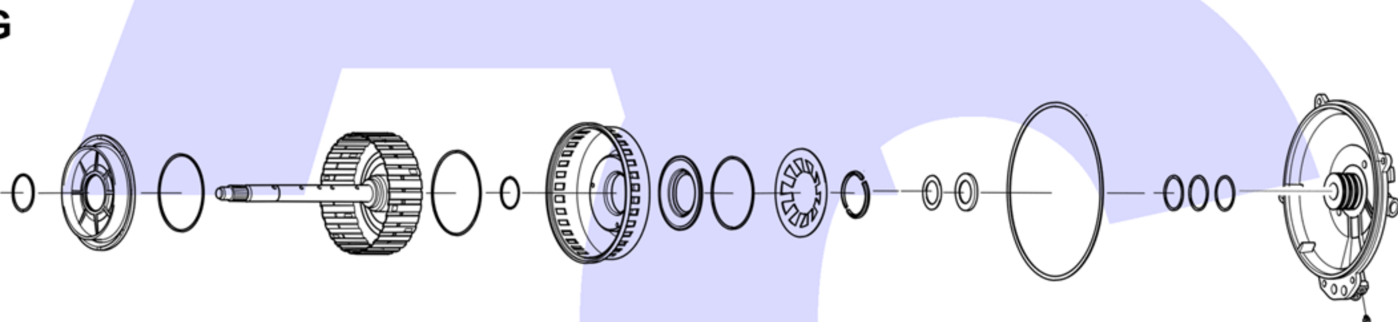
'B' & 'E' Clutch Carriers & End Cover
