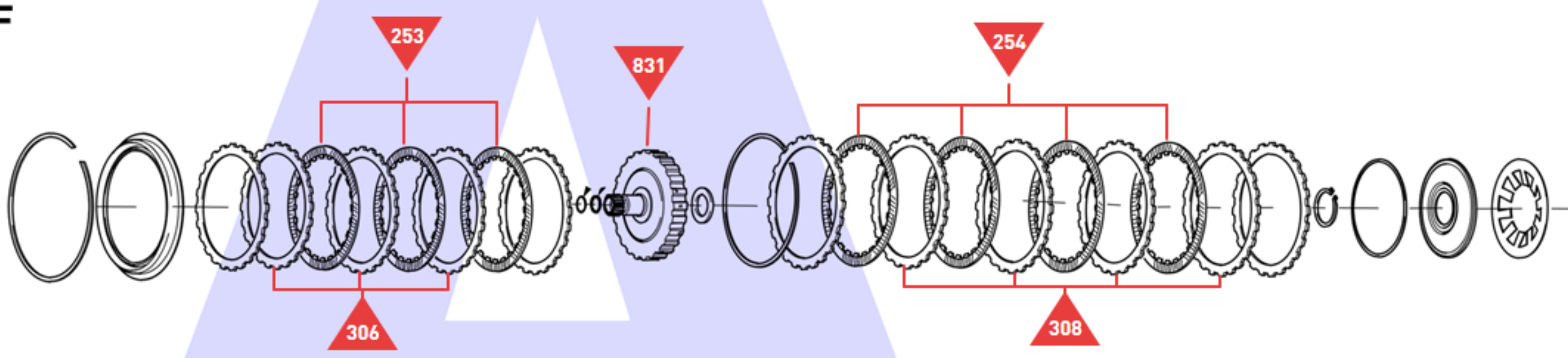
'B' Clutch Assembly
