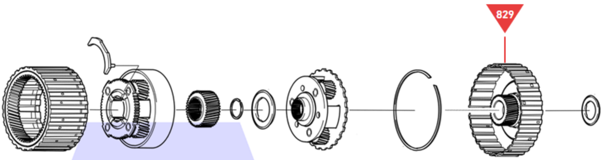
'D' Brake Assembly
