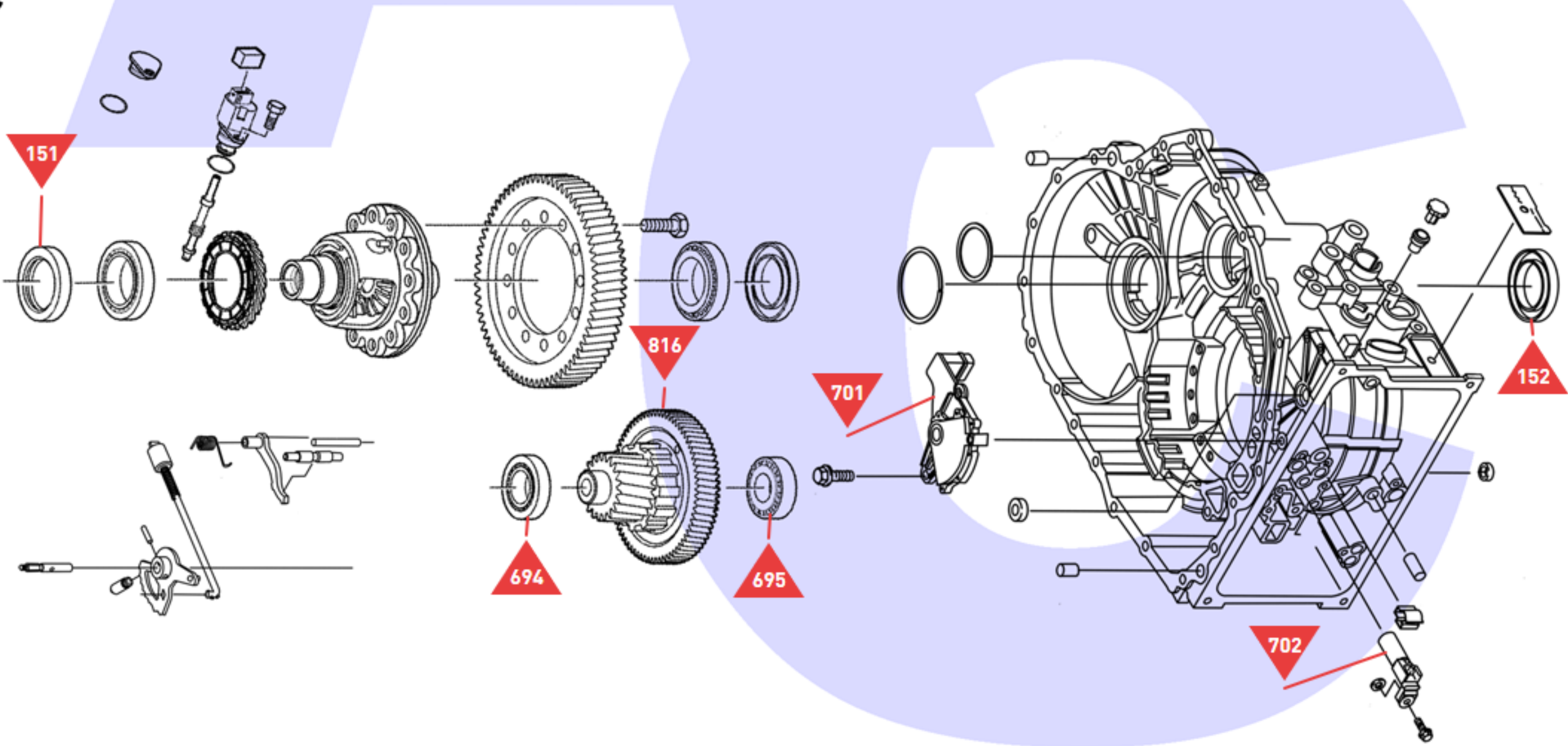
Differential, Main Case & Components
