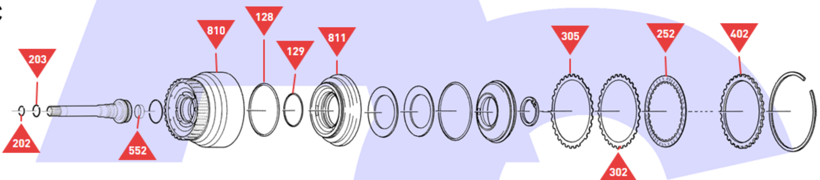
'A' Clutch Assembly
