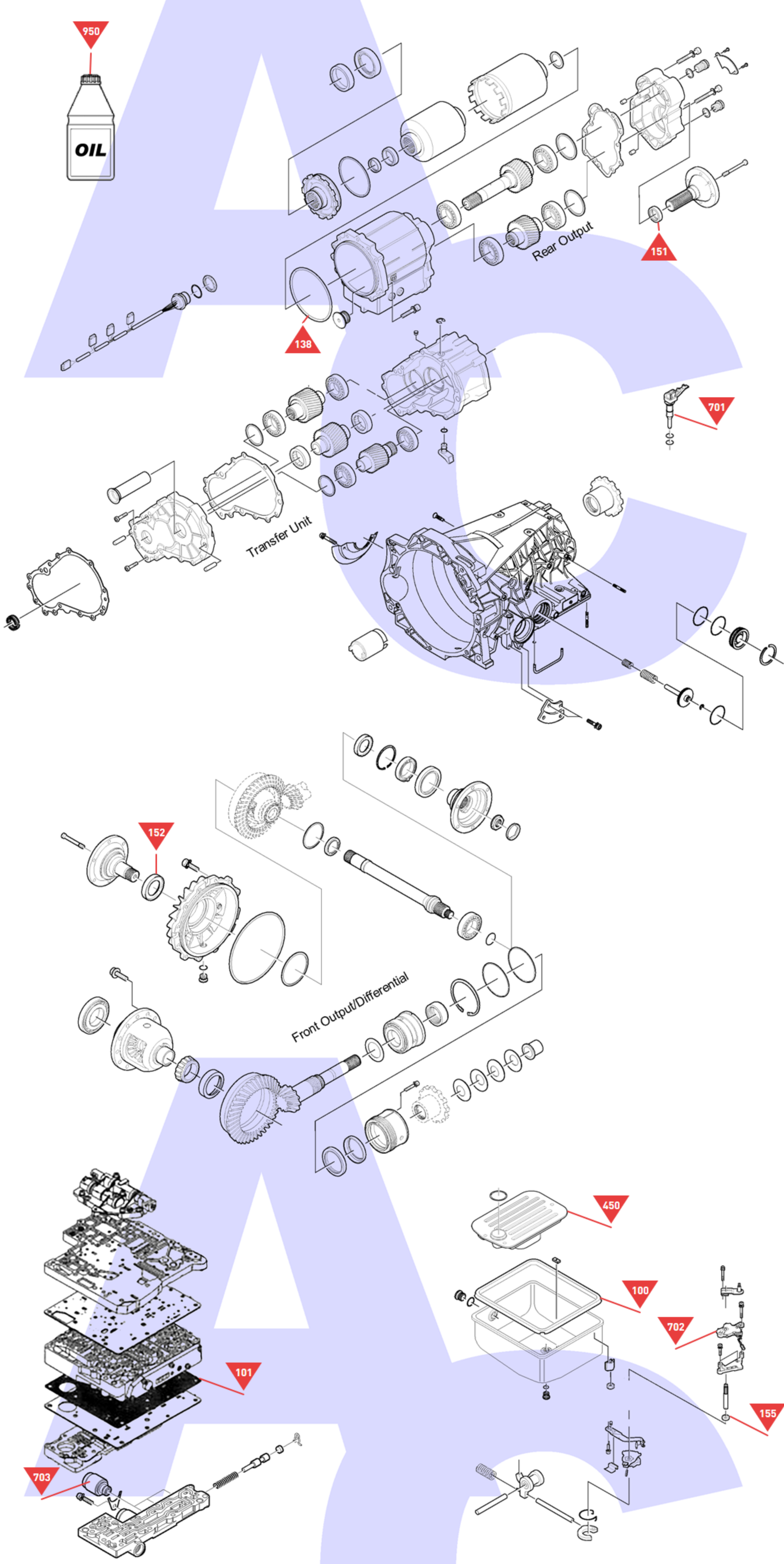
Casing, Output Units, Valve Body, Oil Pan, Filter Etc.
