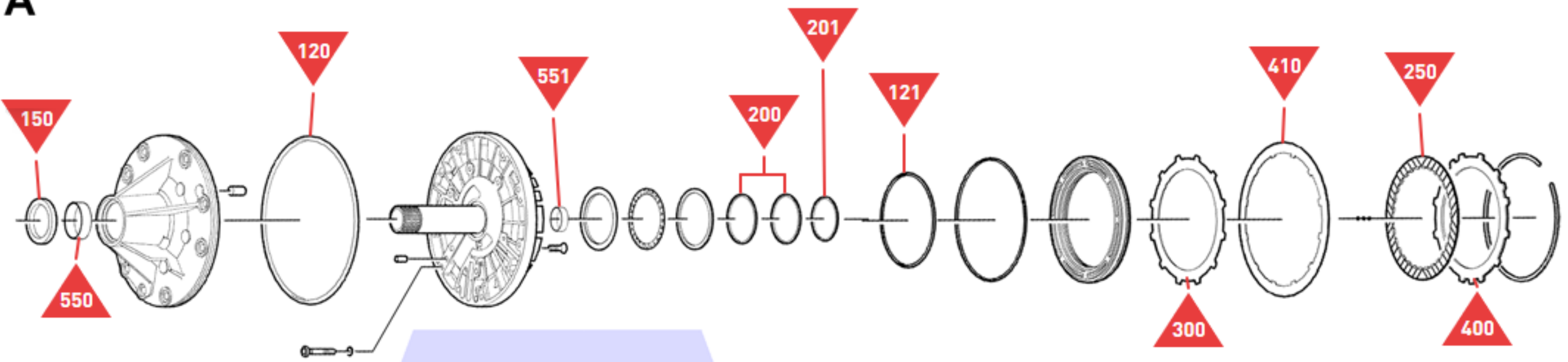
Oil Pump Assembly
