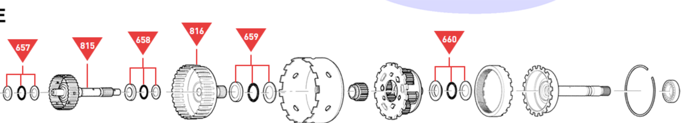
'E' Clutch Assembly
