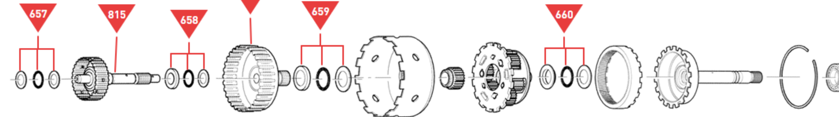
Intermediate Shaft, Sun Gear Shaft, Drive Shell, Planetary Assembly and Output Shaft
