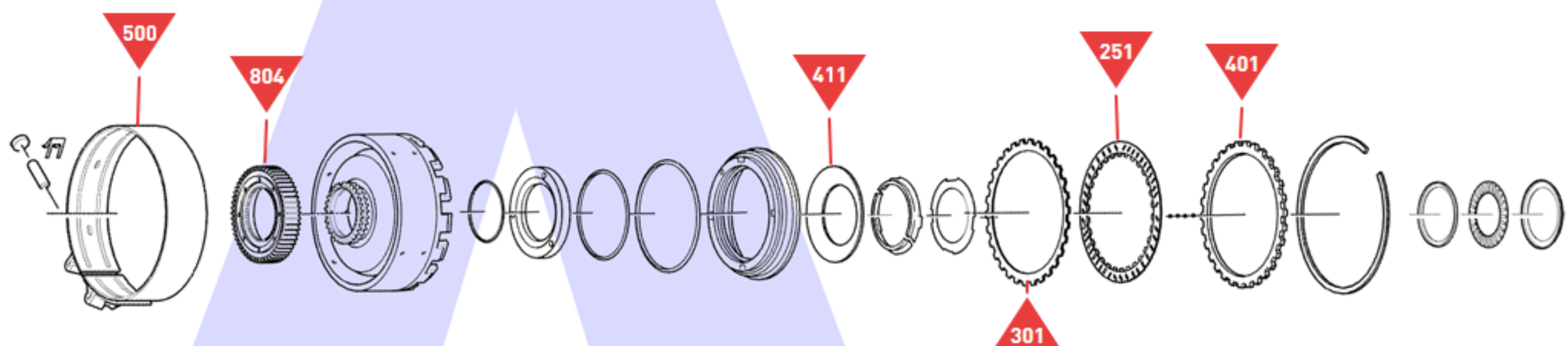
'B' Clutch Assembly
