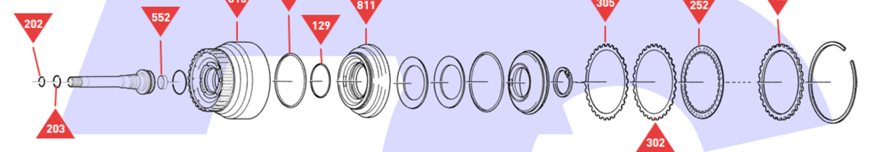
'A' Clutch Assembly
