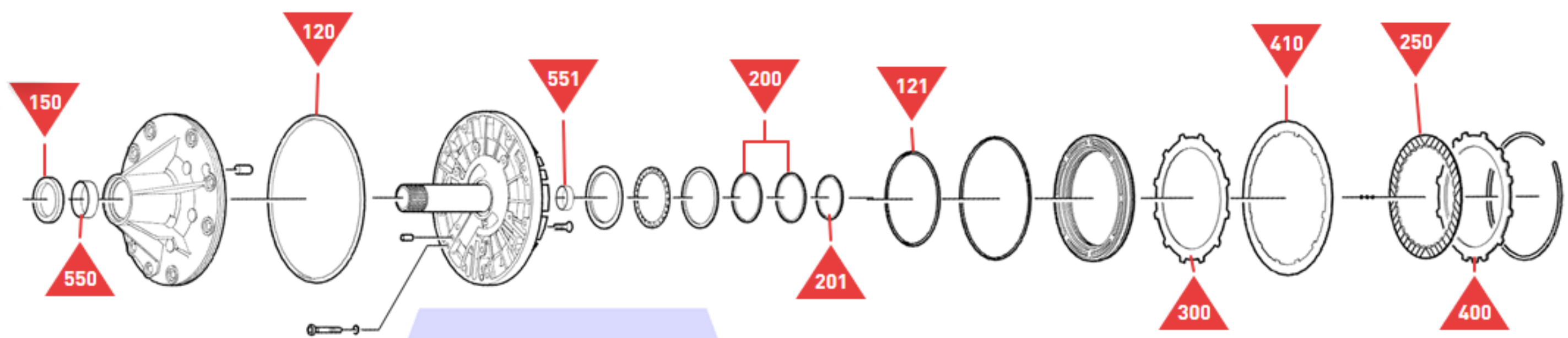
Oil Pump Assembly
