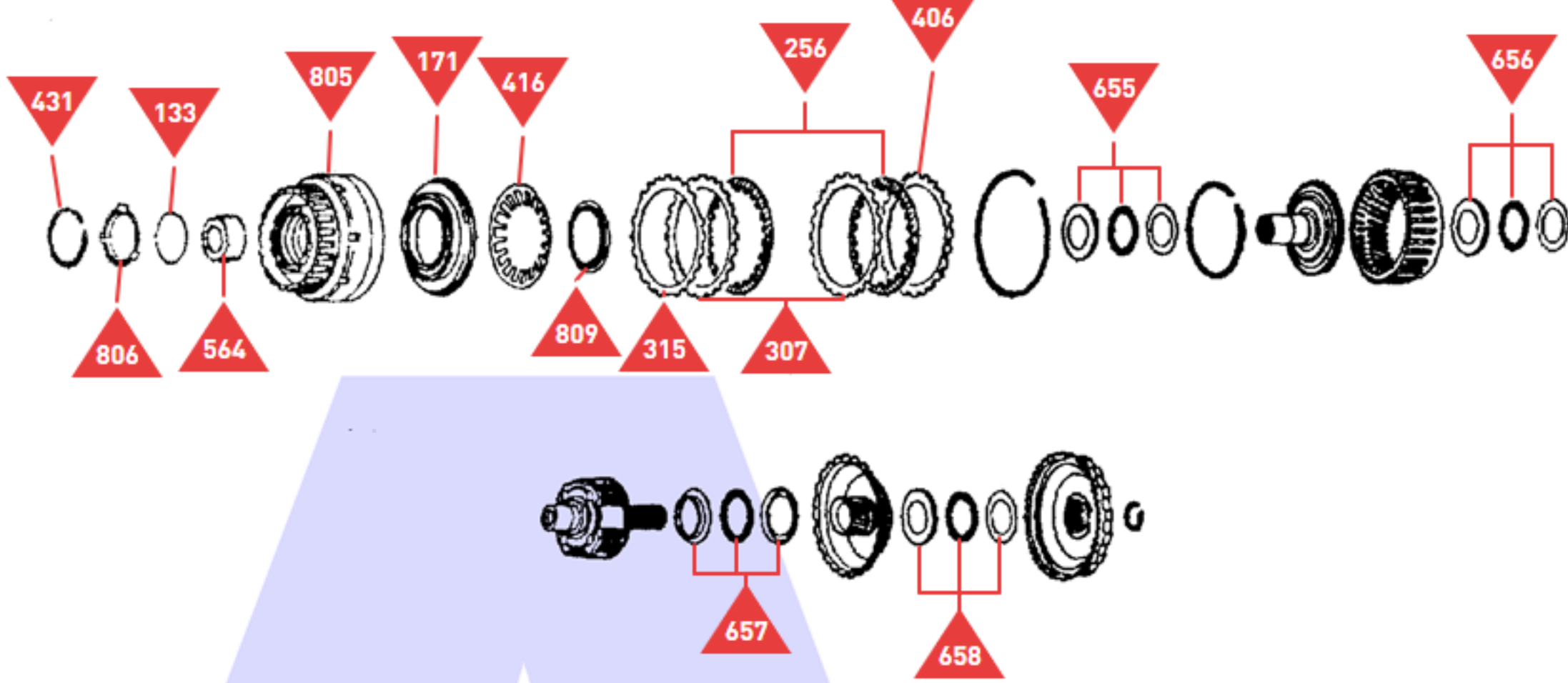
'F' Clutch and Overdrive Planetary
