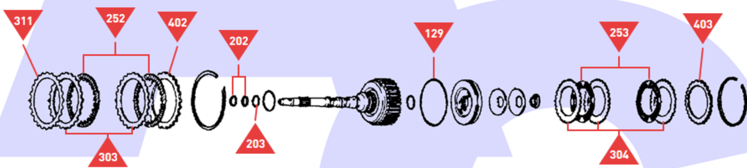
'A' and 'E' Clutches
