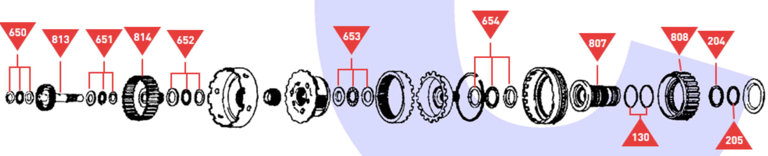
'A' and 'E' Clutches
