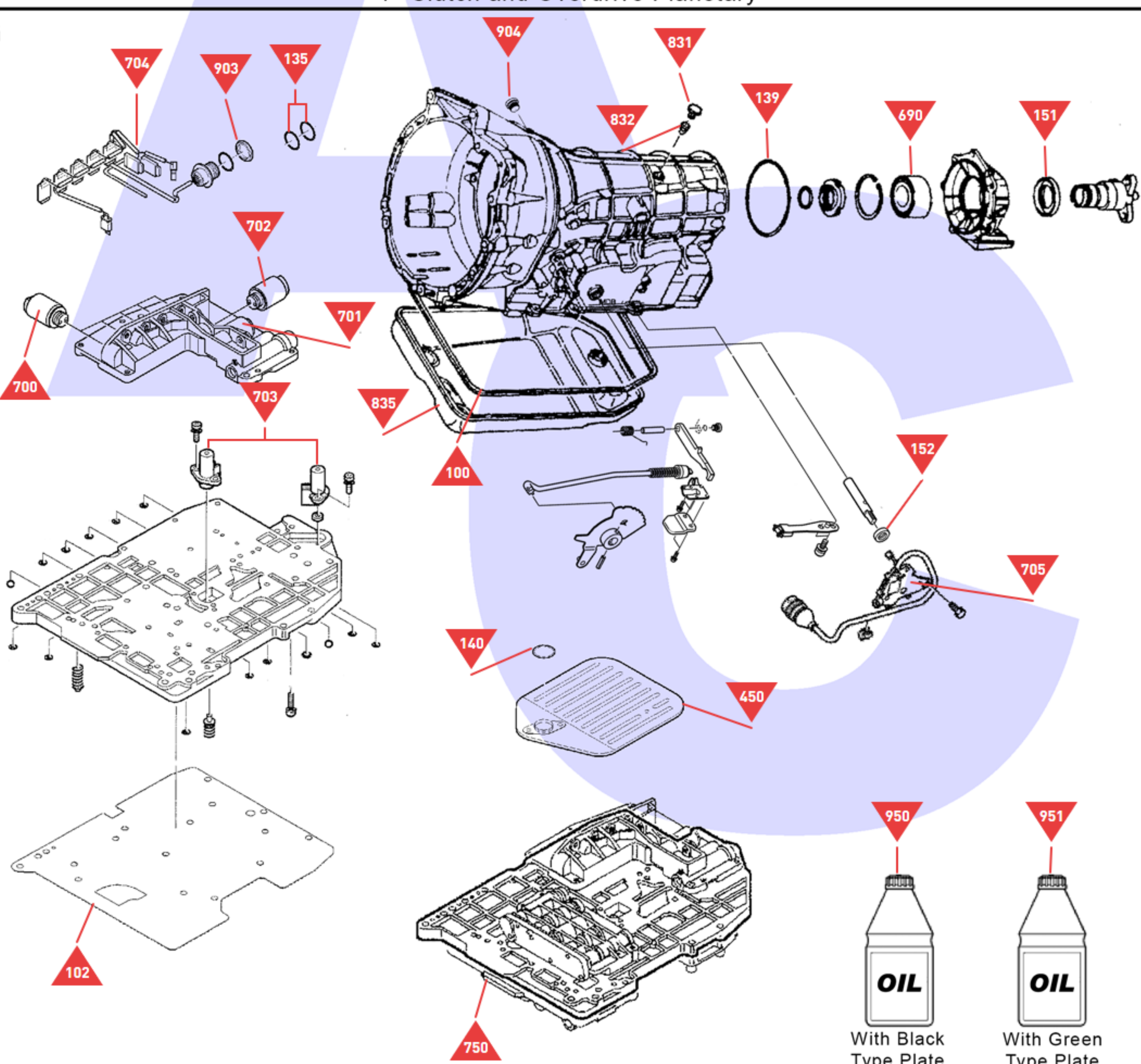
Casings, Valve Body, Filter Etc.
