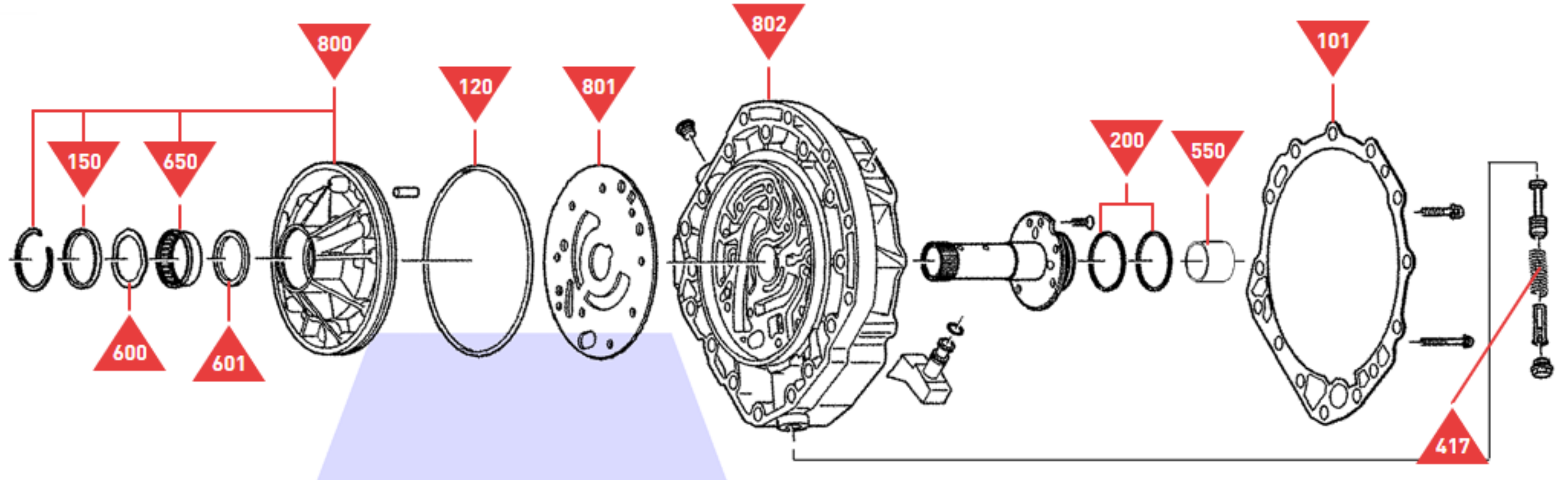
Oil Pump Assy
