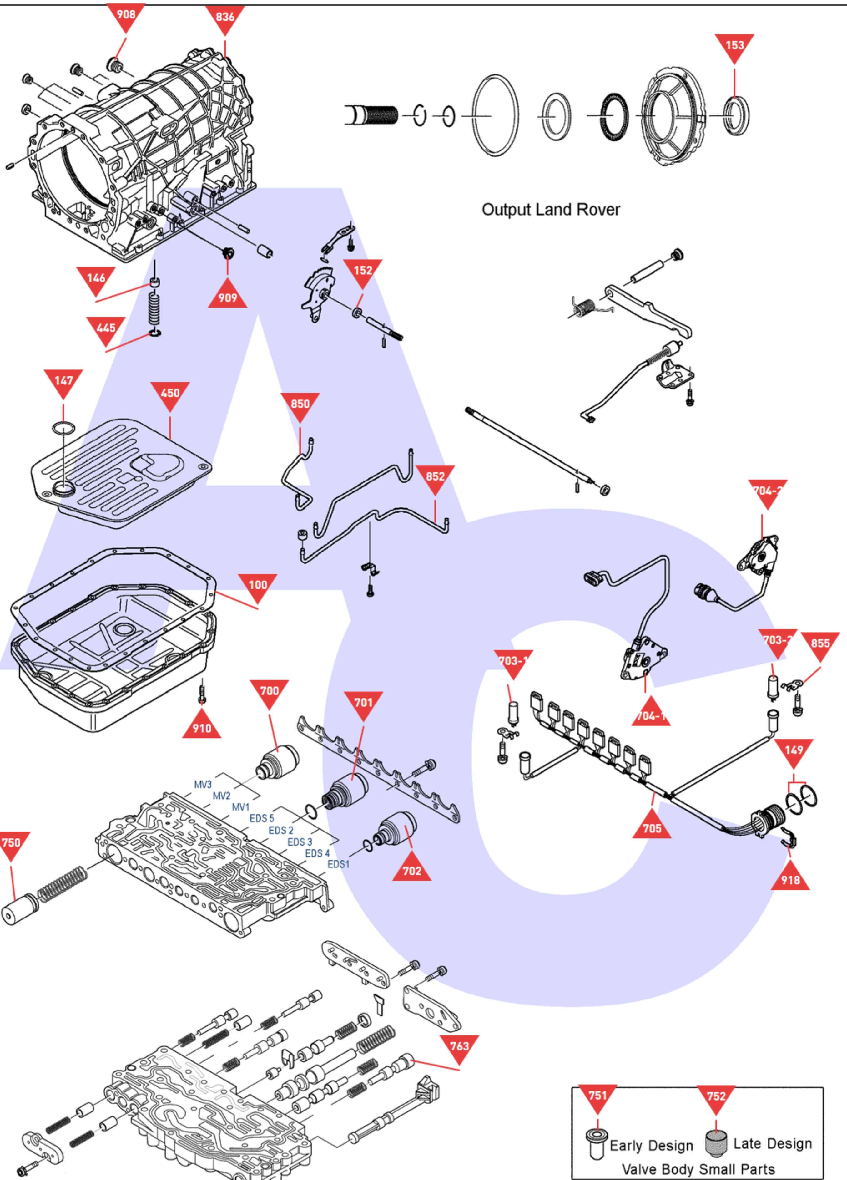
Park Mechanism, Oil Pan, Filter & Electrical Components
