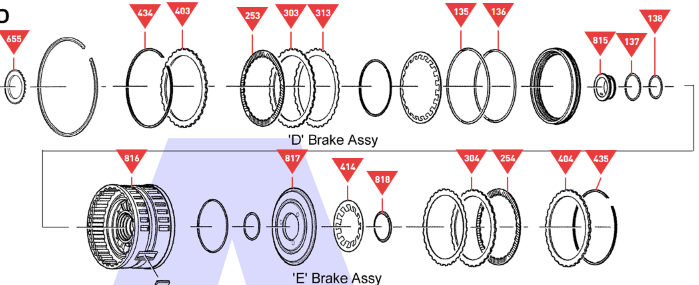
'E' Brake Assy
