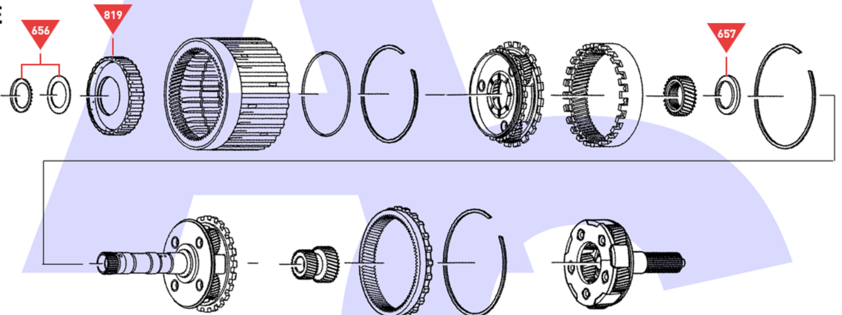
Planetary Assy's
