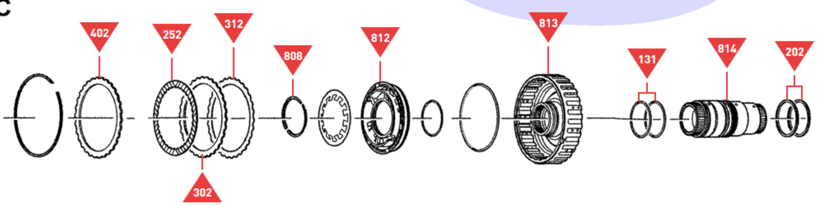
'C' Clutch Assy
