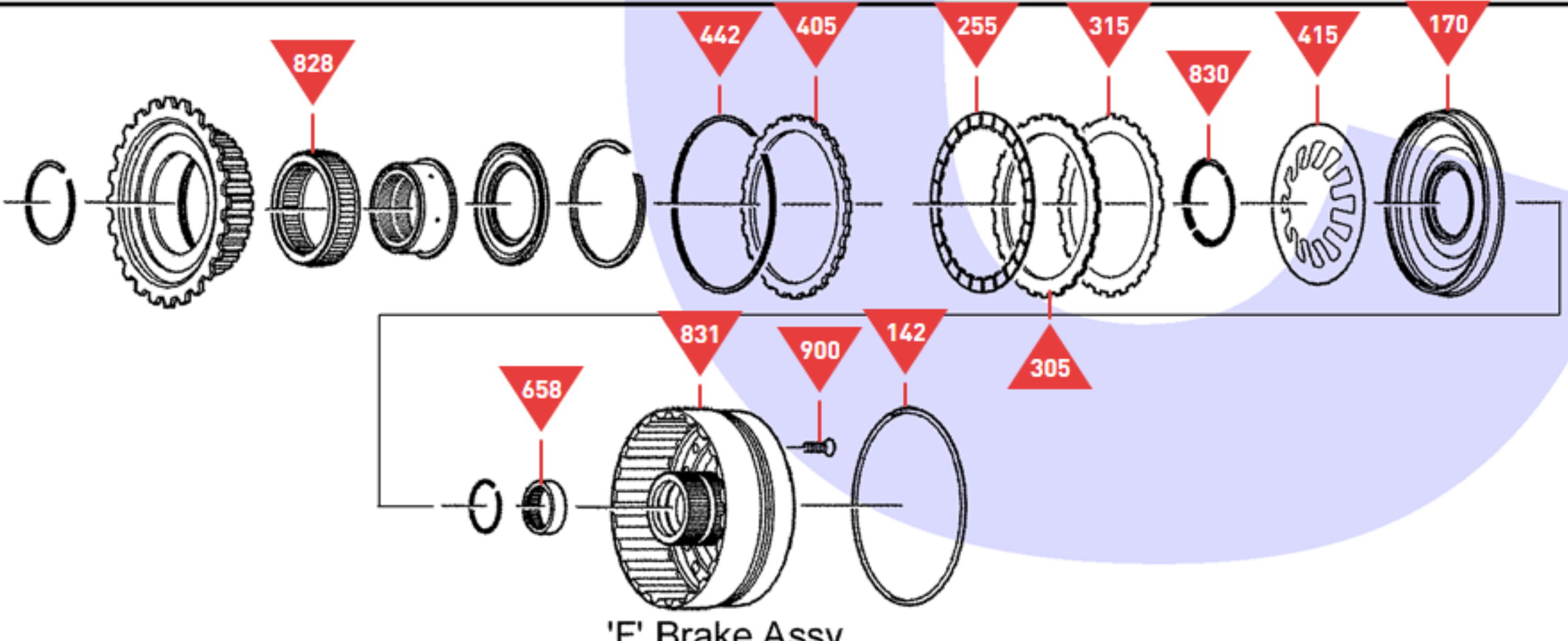
'F' Brake Assy
