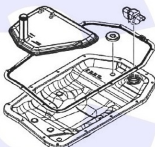
6HP19X Pan Gasket 6HP19.GAS01 Filter 6HP19.FIL03 With Metal Oil Pan
