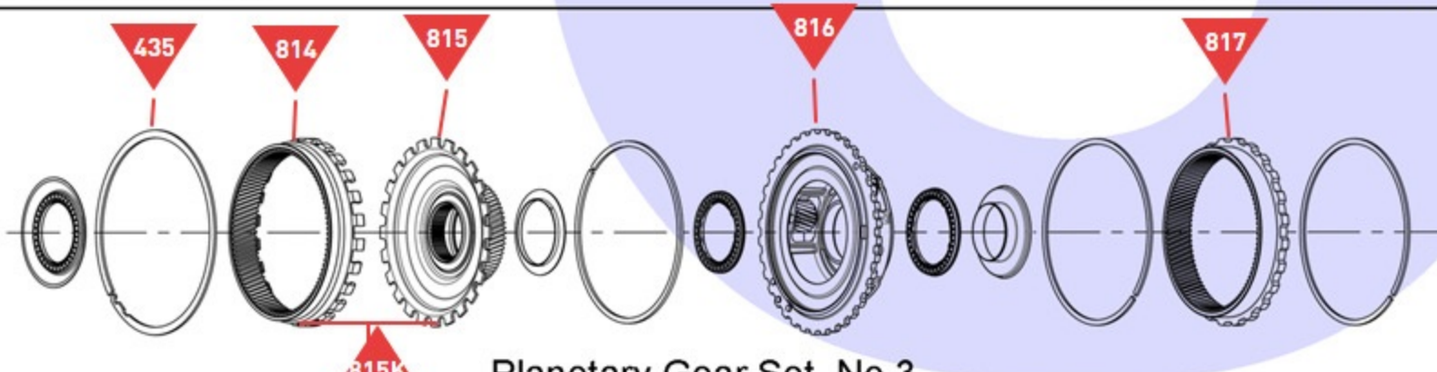
Planetary Gear Set No.3
