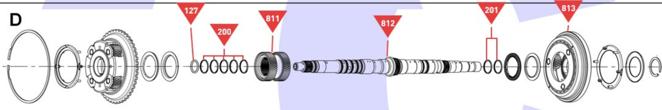
Planetary Gear Set No.1
