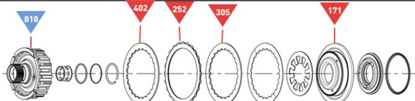
Planetary Gear Set No.3
