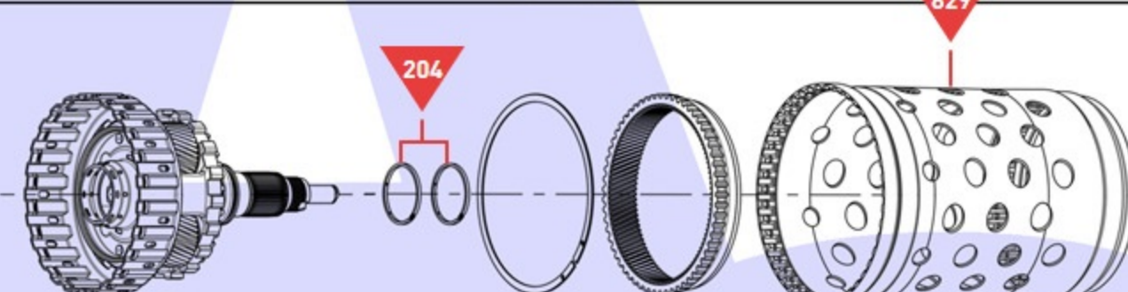
Planetary Gear Set No. 4
