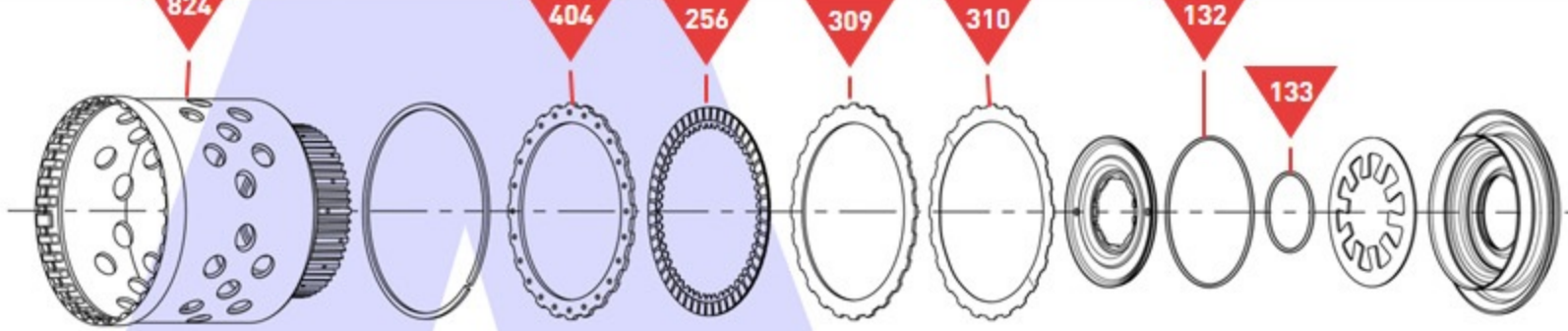
'D' Clutch
