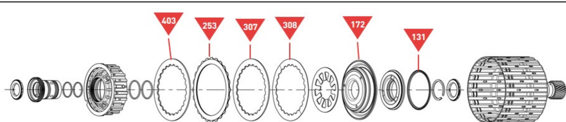
'E' Clutch
