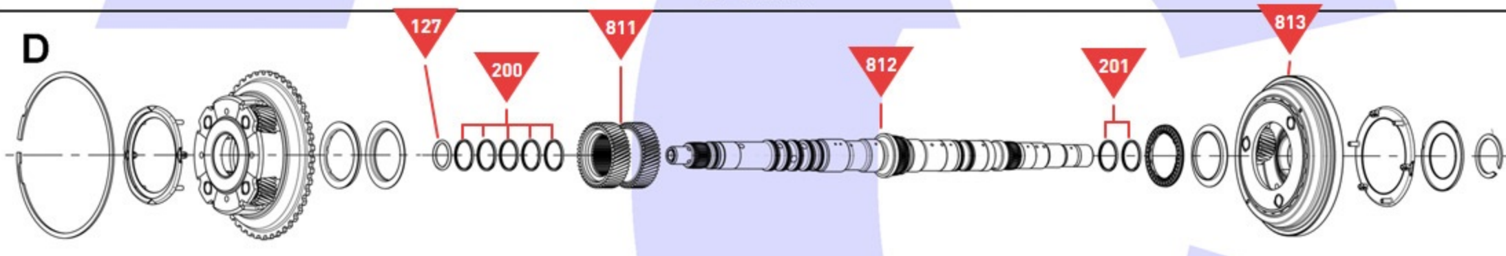
Planetary Gear Set No.1
