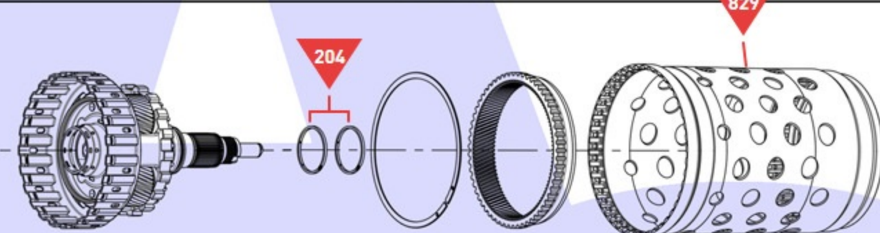
Planetary Gear Set No. 4
