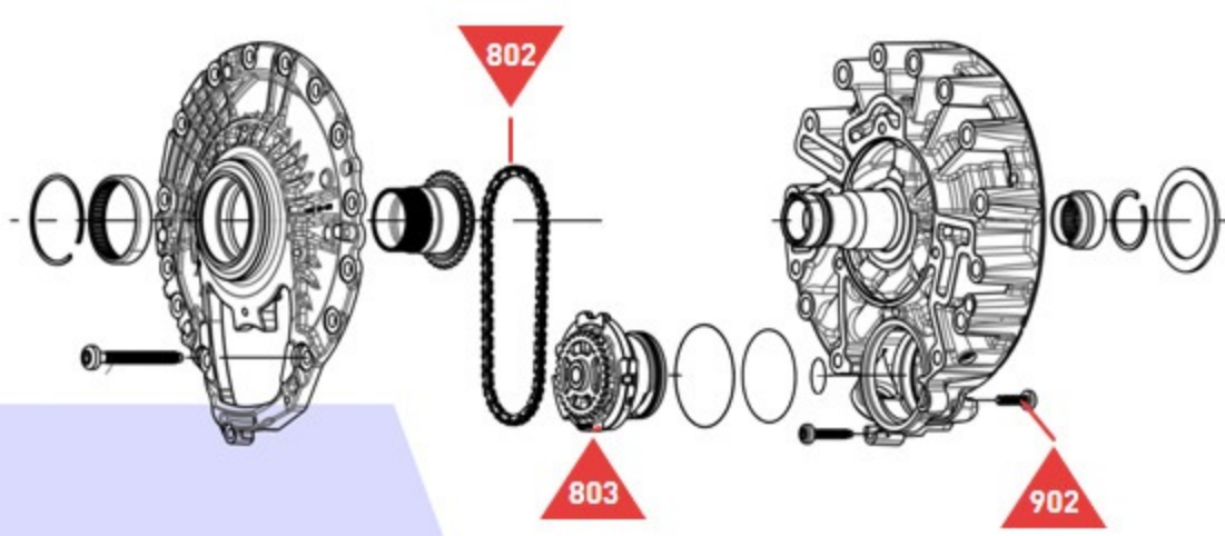
Oil Pump
