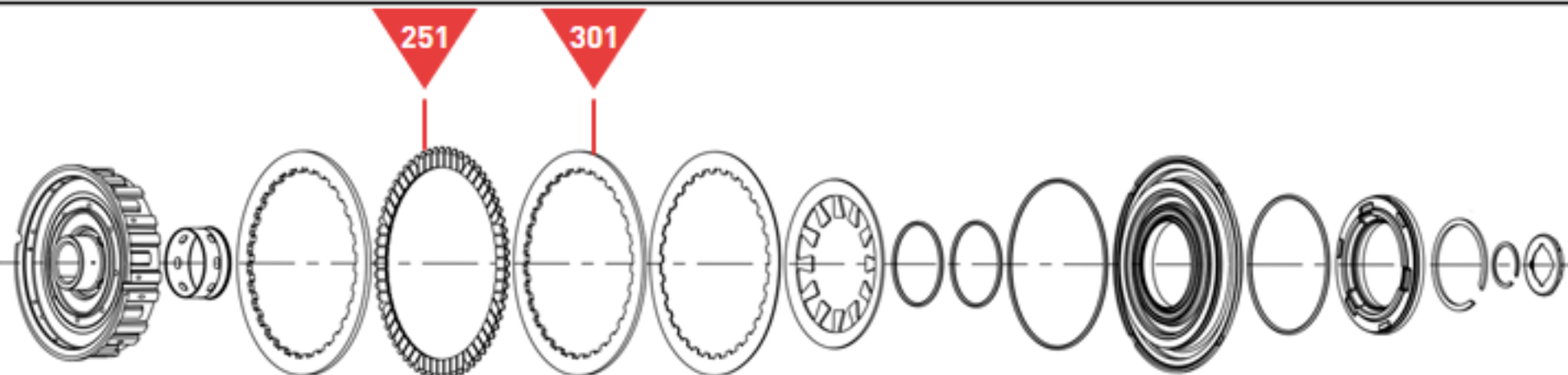
Remaining Input & Planetary with Dog Clutch 'A'
