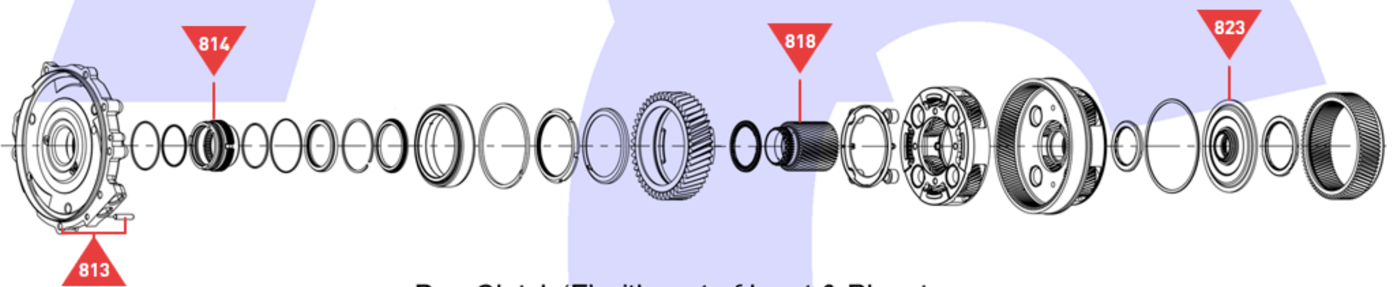
Dog Clutch 'F' with part of Input & Planetary
