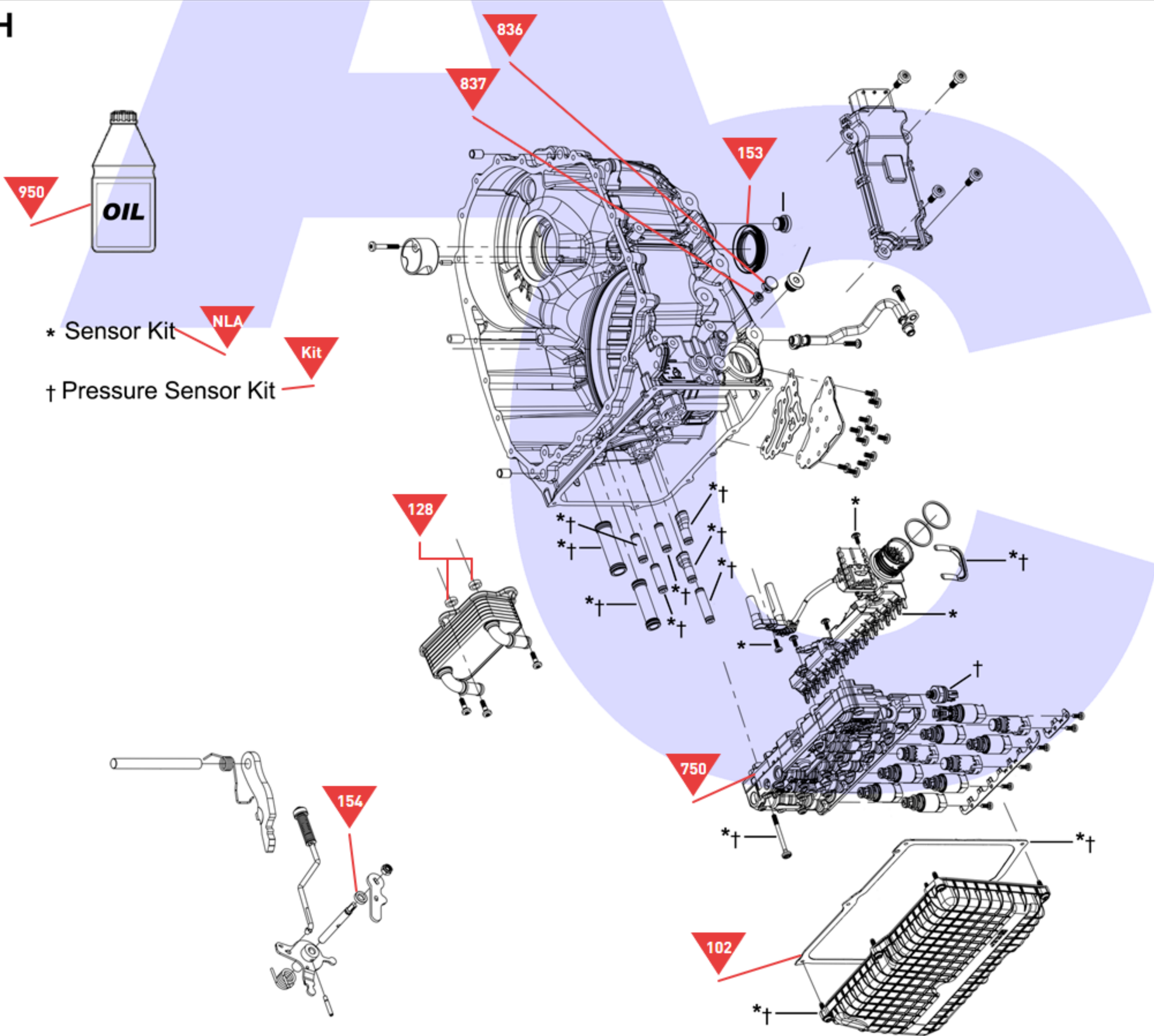
Main Case, Cooler, Valve Body & Control Unit Etc.
